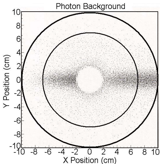
Figure 5.4: GEANT simulation of photon flux at the lumi.
