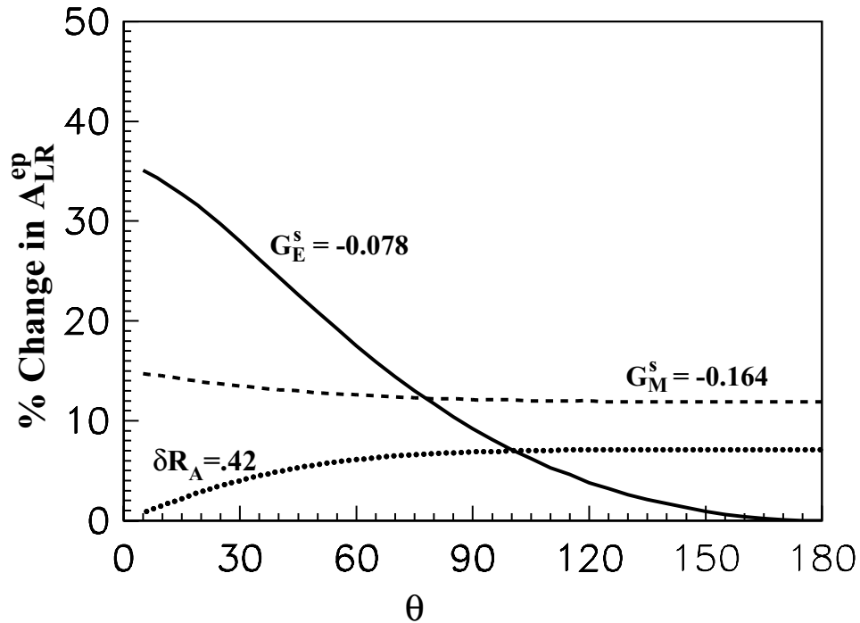
Figure 2.2: Fractional change in A_{LR}^{ep} due to nonzero strange form factors as a function of lab-frame scattering angle evaluated at Q^2 = 0.25 \text{ GeV}^2 . The solid curve shows the effect of G_E^s = -0.078 , the dashed curve shows the effect of G_M^s = -0.164 , and the dotted curve shows the effect of the axial radiative correction, assuming \delta R_A = 0.42 .
