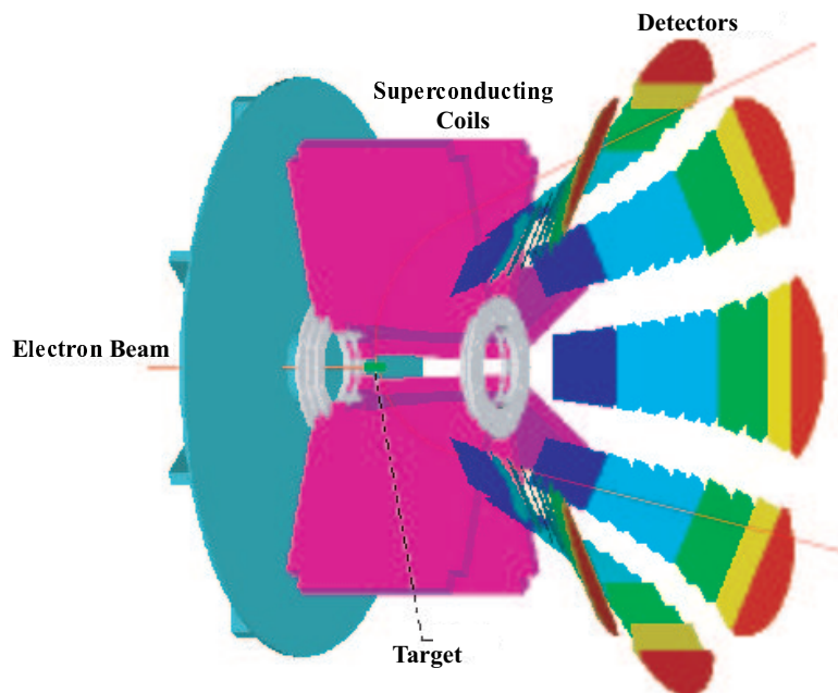
Figure 8.5: Schematic of the G0 experimental setup configured for the forward-angle measurement. The electron beam, incident from the left, strikes a liquid hydrogen target (green, center). Ejected protons are momentum-analyzed by a superconducting magnet and strike an array of scintillator paddles. Each scintillator paddle thus defines a bin in Q^2 .
