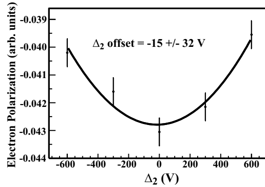
Figure 6.12: Electron beam polarization as a function of PS cell offset \Delta_2 . The CP cell offset \Delta_1 = 0 V. A parabola is fit to the data to approximate the \cos(\frac{\pi\Delta_2}{V_{\lambda/2}}) dependence for \Delta_2 \ll V_{\lambda/2} .
