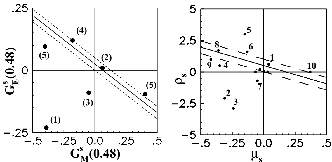
(a) Constraints imposed by this measurement on G_E^s + 0.392G_M^s . The solid line is the result, and the dashed lines are the one-sigma errors. The black points are theoretical predictions arising from various models: (1) [20], (2) [22], (3) [124], (4) [25], and (5) [26].
