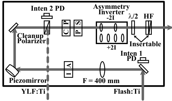
Figure 6.5: The Helicity Control Bench contains the optics for control of the laser beam's polarization and \text{beam}_{\text{A}_{\text{LR}}} 's.
