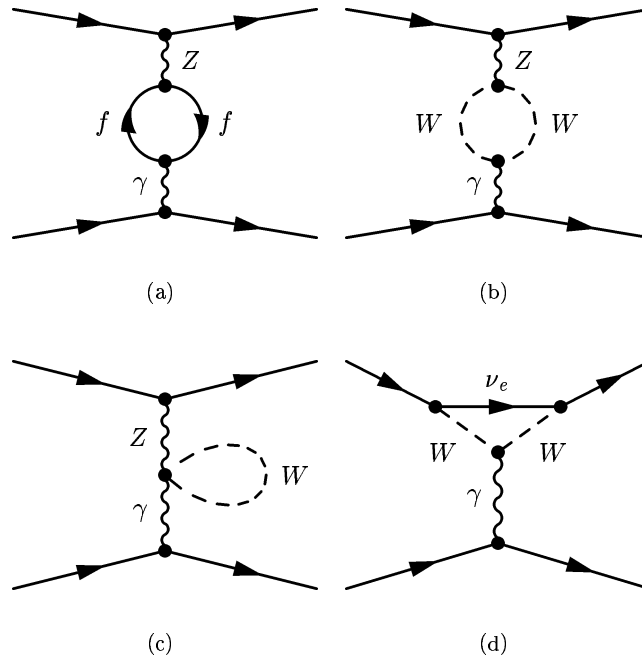
Figure 2.7: \gamma - Z mixing diagrams (a-c) and the W -loop contribution to the anapole moment (d). Inverted and crossed diagrams contribute as well.
