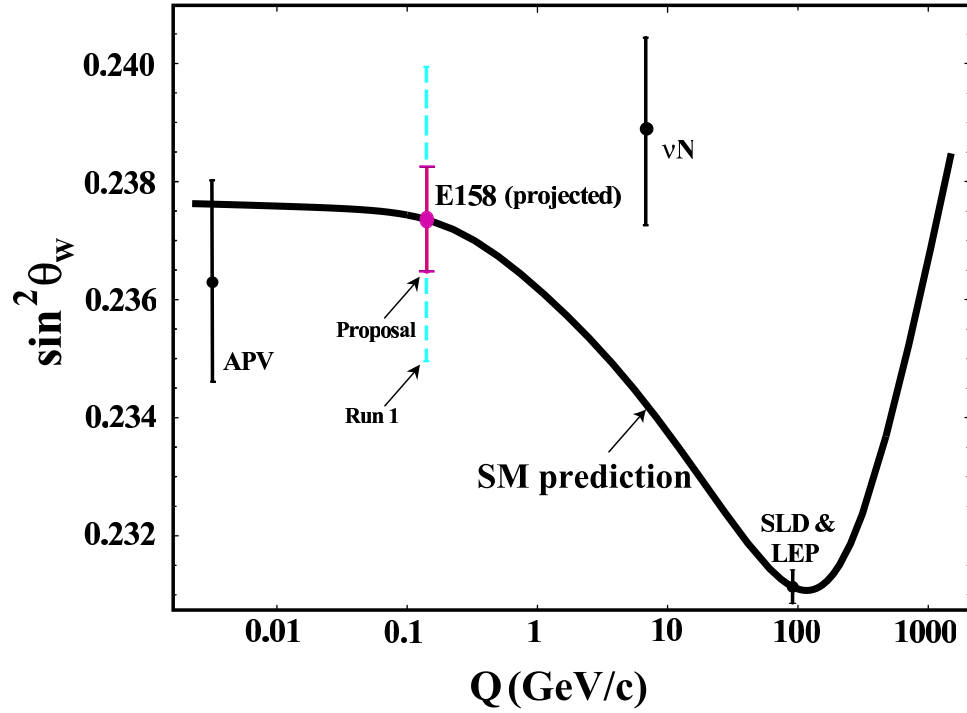
Figure 2.6: Running of \sin^2 \theta_W from the precision measurement at the Z^0 resonance as predicted by the Standard Model (Adapted from [68]). The NuTeV result is from [65] and the atomic PV result is from [66, 67]. The E-158 results are projected results for Run I (completed April-May, 2002) and for the proposal goal.
