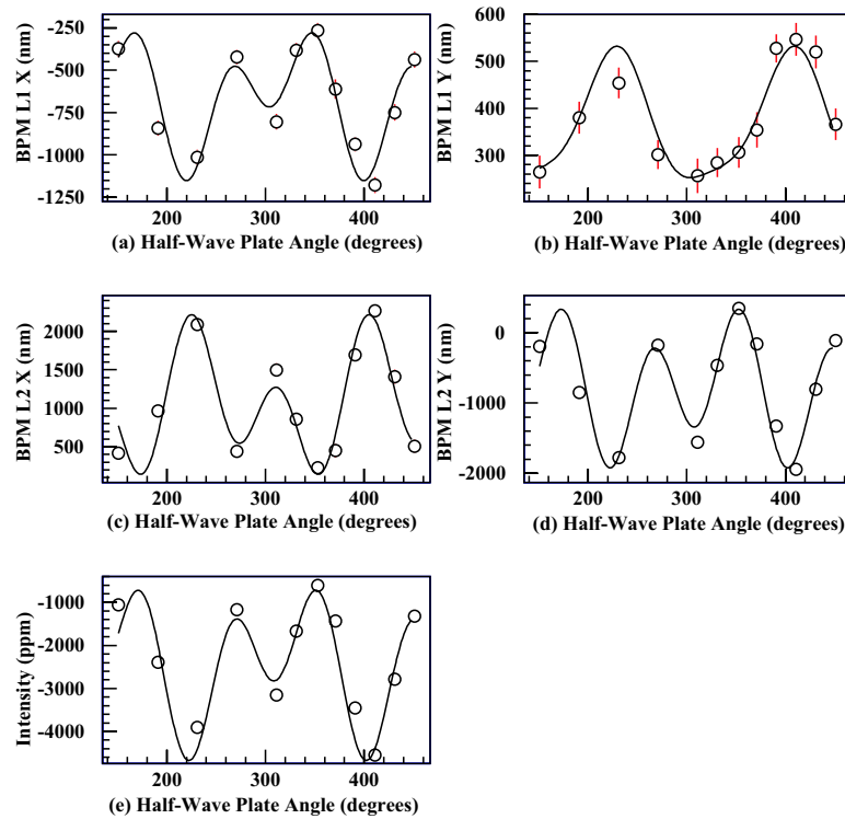
Figure 4.12: Dependence of position differences measured by two BPM's at the 5-MeV point in the Injector (a-d) on the orientation of the rotatable half-wave plate. The position differences show a strong correlation with the intensity asymmetry (e).
