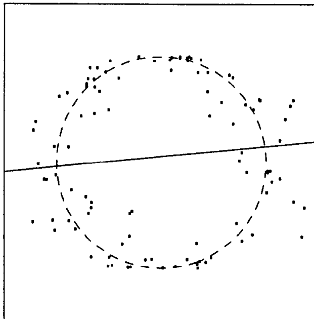
Figure 3.7b The dashed curve is the principal component line. D(\hat{f}^{(0)}) = 3.43
