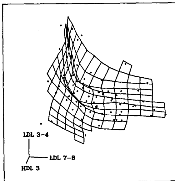
Figure 6.6d The principal surface as in figure 6.6a from a slightly oblique perspective.
