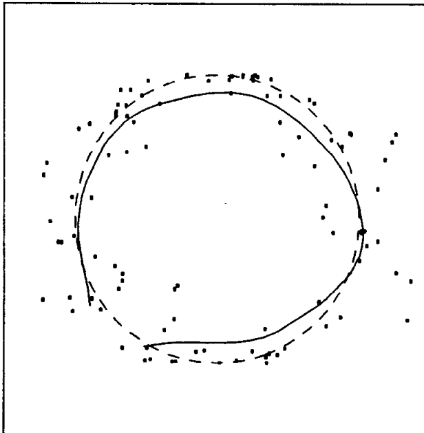
Figure 3.7k D(\hat{f}^{(9)}) = 0.97 . The span is automatically reduced at this stage.
