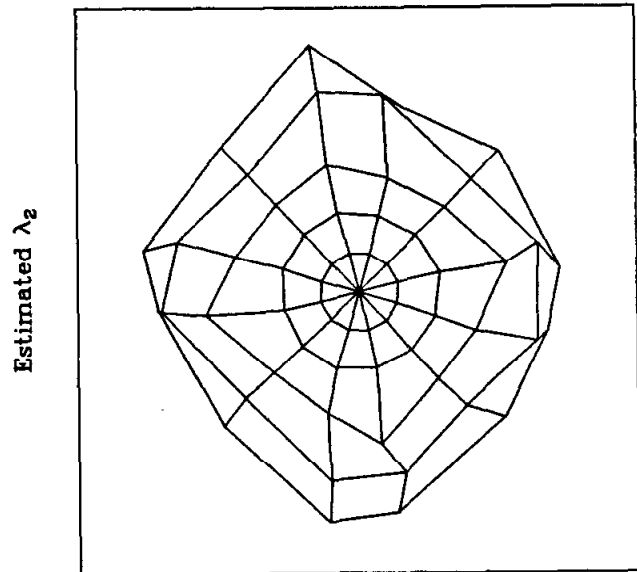
Estimated \lambda_1
