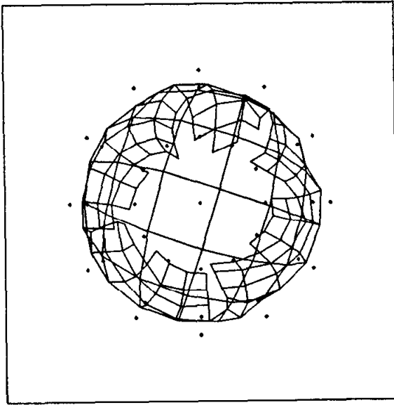
Figure 6.4e Another view of the final principal surface.
