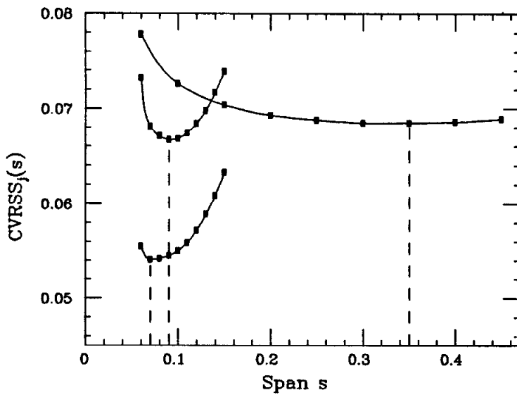
Figure 6.2e The cross-validation curve shows CVRSS_j(s) as a function of the span s . A separate span is found for each co-ordinate.
