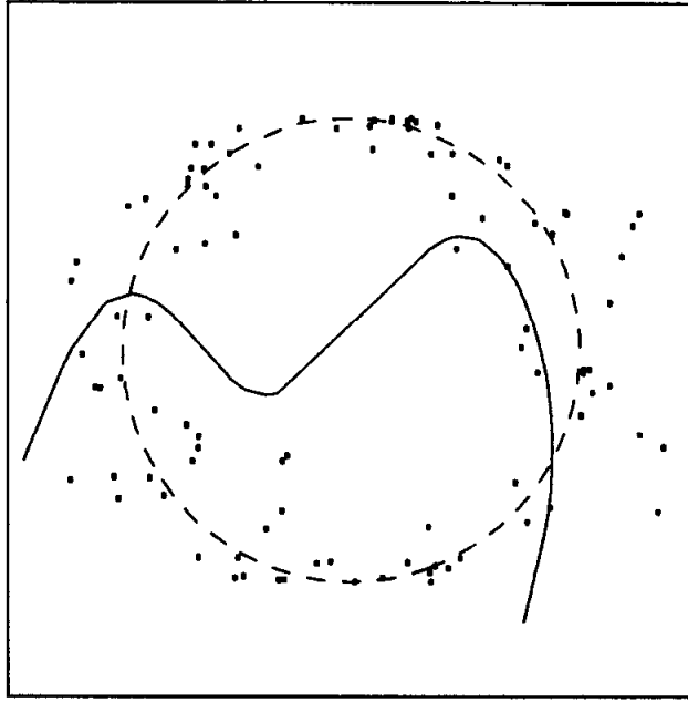
Figure 3.7f D(\hat{f}^{(4)}) = 2.37
