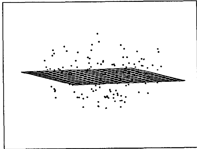
Figure 3.9b. The principal component plane. D(\hat{f}^{(0)}) = 1.59
