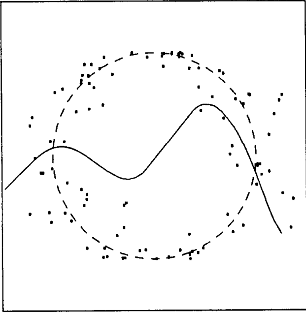
Figure 3.7e D(\hat{f}^{(3)}) = 2.64
