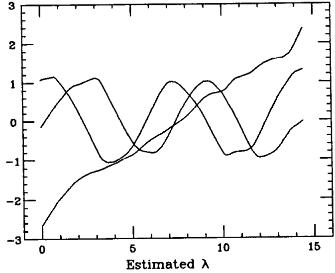
Figure 6.2d The estimated co-ordinate functions for the helix, using the span found in figure 6.2c.
