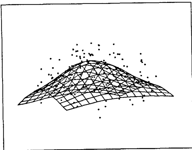
Figure 3.9c. D(\hat{f}^{(1)}) = 1.20
