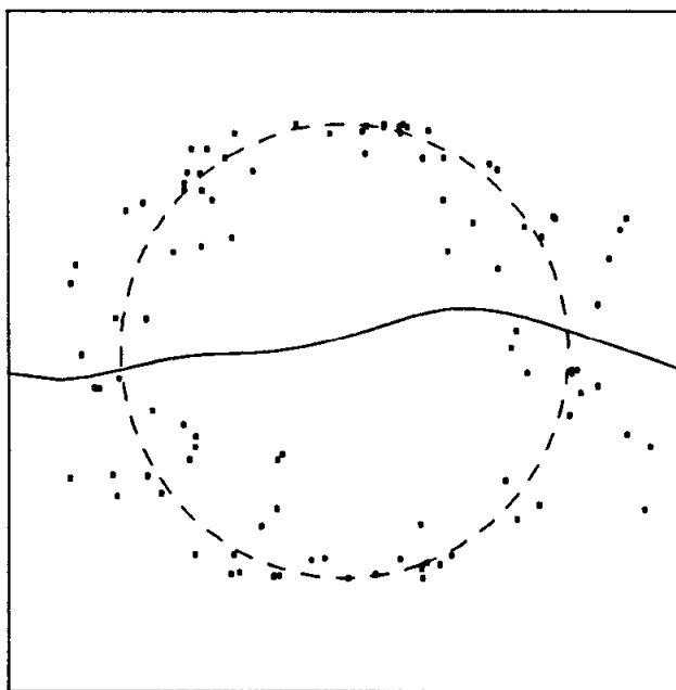
Figure 3.7c D(\hat{f}^{(1)}) = 3.34
