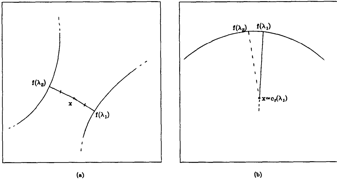
Figure 3.4 The continuity constraint avoids global ambiguities (a) and local ambiguities (b) in projection.
