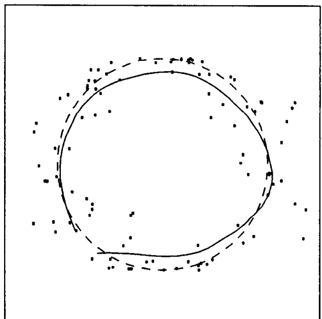
Figure 3.7l D(\hat{f}^{(10)}) = 0.96
