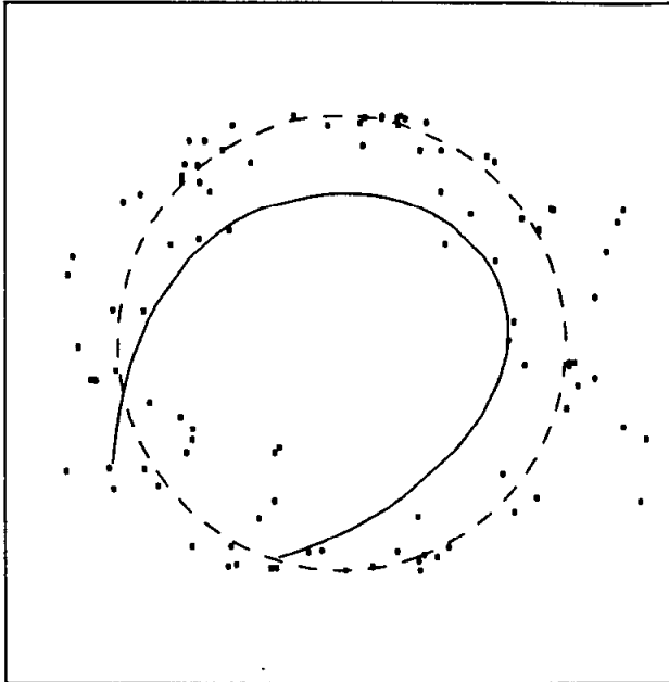
Figure 3.7i D(\hat{f}^{(7)}) = 1.64
