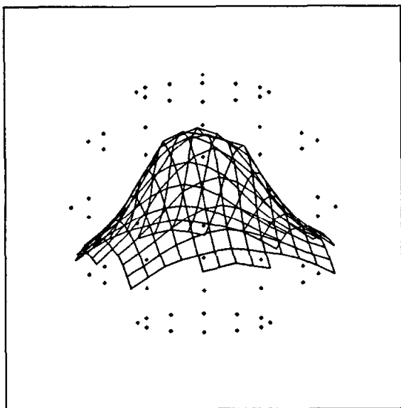
Figure 6.4c An intermediate stage in the iterations.
