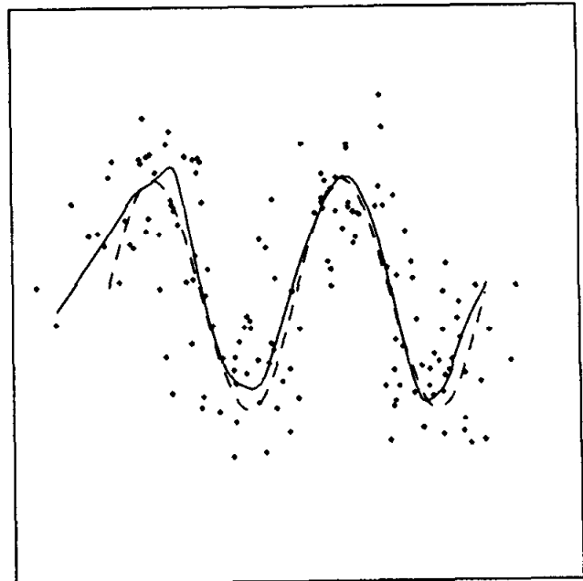
Figure 6.2b Another view of the helix, the data and the principal curve.
