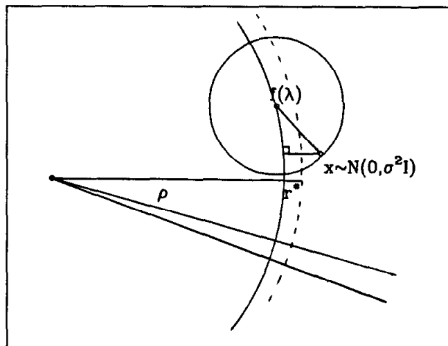
Figure 4.5 The data is generated from the arc of a circle with radius \rho and with iid \mathcal{N}(0, \sigma^2 I) errors. The location on the circle is selected uniformly.
