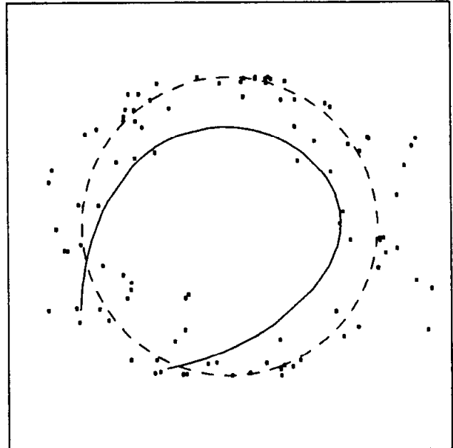
Figure 3.7j D(\hat{f}^{(8)}) = 1.60
