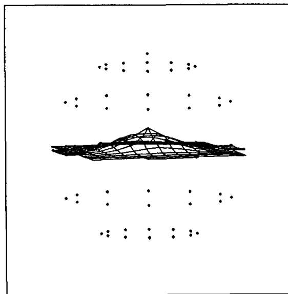
Figure 6.4b The second iteration of the principal surface procedure finds a surface that is a function of the first iteration.
