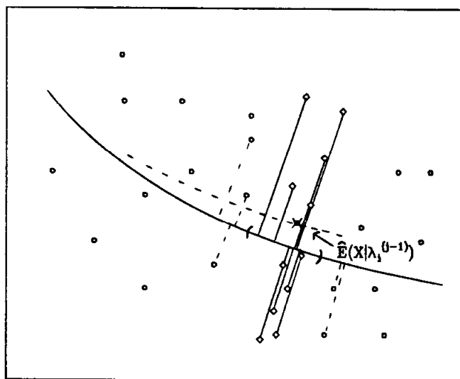
Figure 3.6 We estimate the conditional expectation \mathbf{E}(X | \lambda^{(j-1)} = \hat{\lambda}_i^{(j-1)}) by averaging the observations \mathbf{x}_k for which \hat{\lambda}_k^{(j-1)} is close to \hat{\lambda}_i^{(j-1)} .
