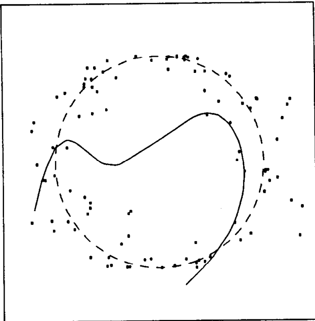
Figure 3.7g D(\hat{f}^{(5)}) = 2.25
