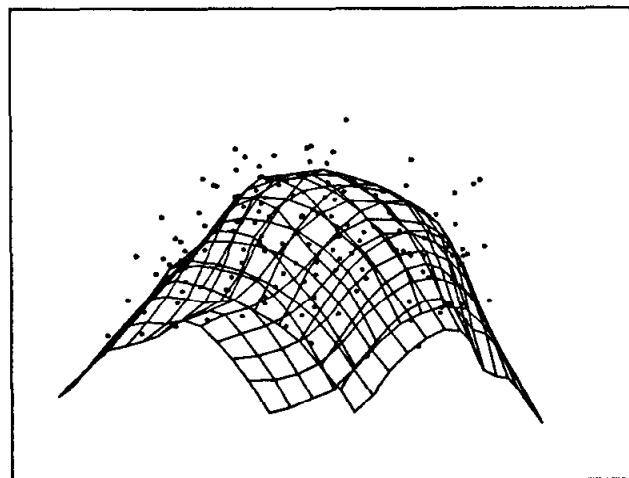
Figure 3.9d. D(\hat{f}^{(4)}) = 0.78
