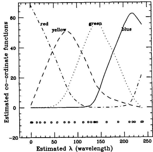
Figure 6.5b The estimated co-ordinate functions plotted against the arc length of the principal curve. This \hat{\lambda} will be monotone with the true wavelength.
