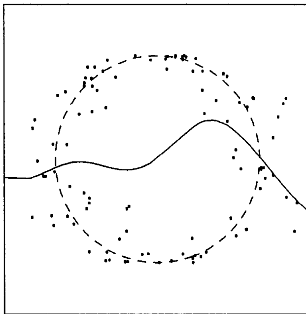
Figure 3.7d D(\hat{f}^{(2)}) = 3.03
