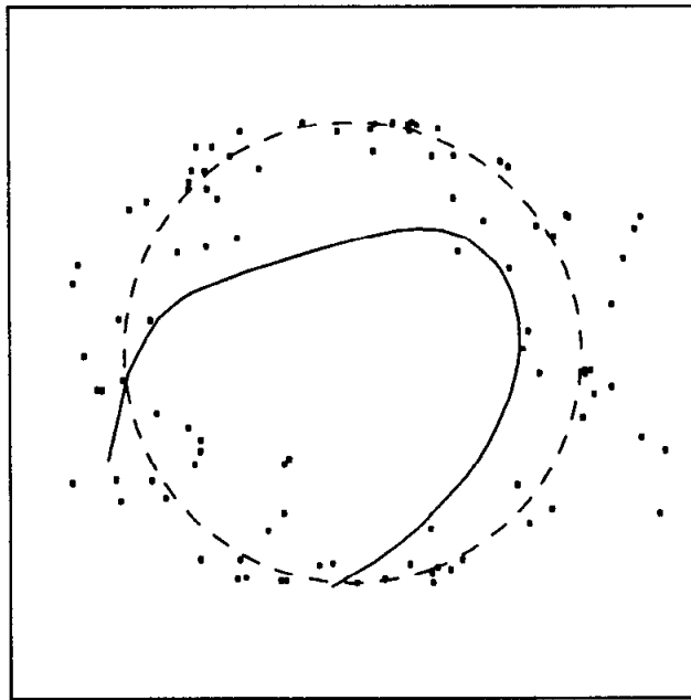
Figure 3.7h D(\hat{f}^{(6)}) = 1.91
