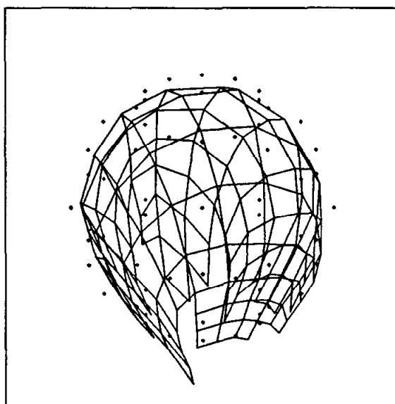
Figure 6.4d The final surface produced by the principal surface routine.
