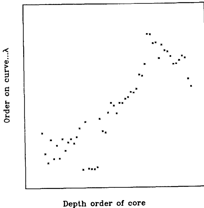
Figure 6.3b The values \lambda_j(x_i) are plotted against the depth order of the core samples.
