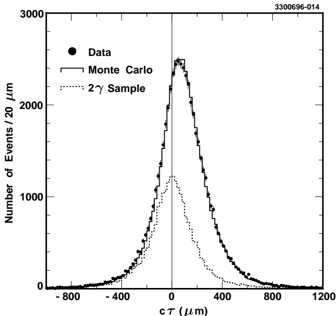
FIG. 1. Decay length distribution for Monte Carlo and Data for 1 vs 3 events. The dashed histogram is for the control sample, discussed in the text, of two-photon events with four charged tracks in the final state.
