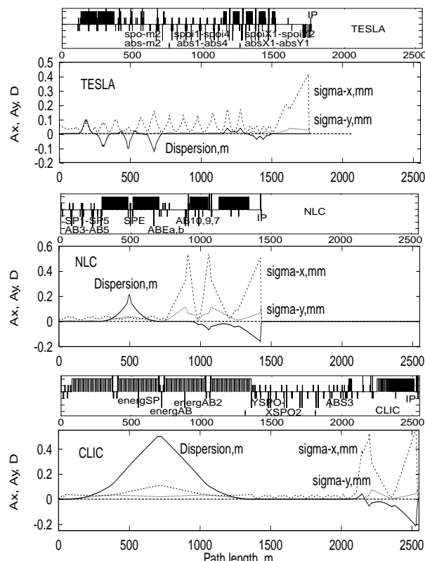
Figure 1: Collimator locations in TESLA, NLC and CLIC. The comparative studies were carried out using the program STRUCT [3]. This package performs particle tracking, taking into account aperture restrictions, interaction of primary beam particles with collimators, beam losses, synchrotron radiation and transport of the photons along the beamline.
