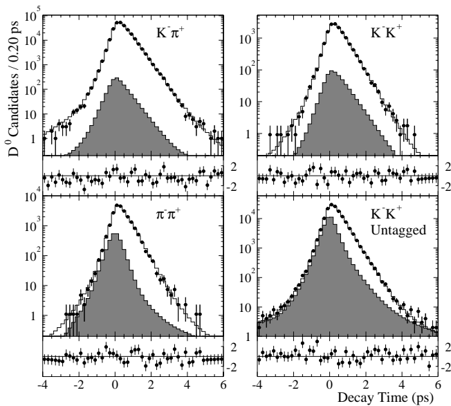
FIG. 2: The decay-time distribution for the four D^0 samples (points) within a \pm 15 MeV/ c^2 mass signal window superimposed on a projection of the lifetime fit (histogram). The shaded histogram is the portion of the sample assigned by the fit to the background. The points presented below the histograms are the difference between data and fit divided by the statistical error with error bars of unit length.
