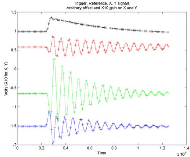
Figure 3: Digitized IF waveforms from the RF cavity BPM's. From top to bottom, the trigger, reference cavity IF and x y IF waveforms are displayed. The time base is in \mu\text{s} .
