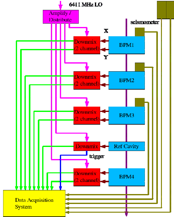
Figure 2: Schematic of the high resolution BPM test equipment, showing the BPM placement along the beamline and the signal processing electronics. In this experiment seismometer vibration monitors (shown on the right) were used to check the motion of the BPM's and BPM supports.
