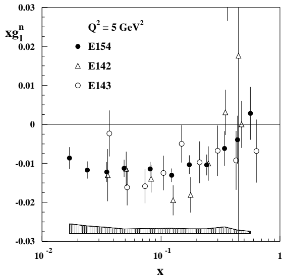
Fig. 9. The E154 results on the structure function xg_1^n (closed circles) compared to the E142 (open triangles) and E143 (open circles) data.
