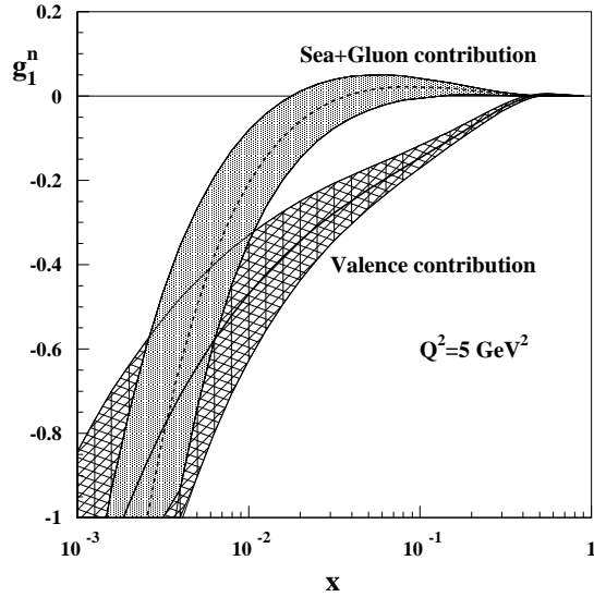
Fig. 13. The contributions to the structure function g_1^n of the neutron from the valence quarks (solid line) and from the sea quarks and gluons (dashed line). The shaded and hatched areas represent the total uncertainties on each quantity.
