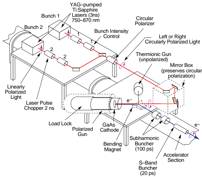
Fig. 4. A schematic of the polarized source at SLAC. The setup shown is for the SLC operation. The E154 setup was very similar, with one of the lasers changed to a flashlamp-pumped Ti:sapphire.
