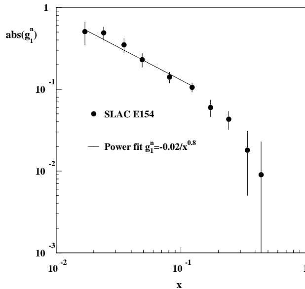
Fig. 10. The absolute value of structure function g_1^n is plotted on a log-log scale. The low- x data points of E154 are fitted with a power-law function g_1 \sim x^{-0.8} .
