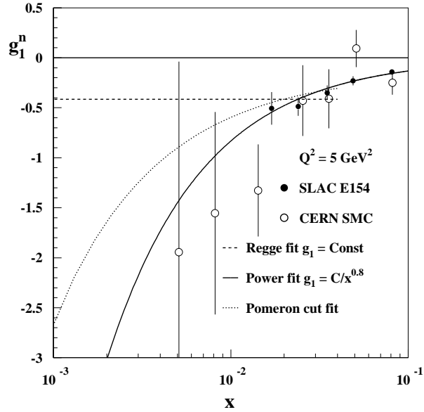
Fig. 11. Three representative fits to the low- x data of E154. Also included are the low- x data of SMC (open circles).
