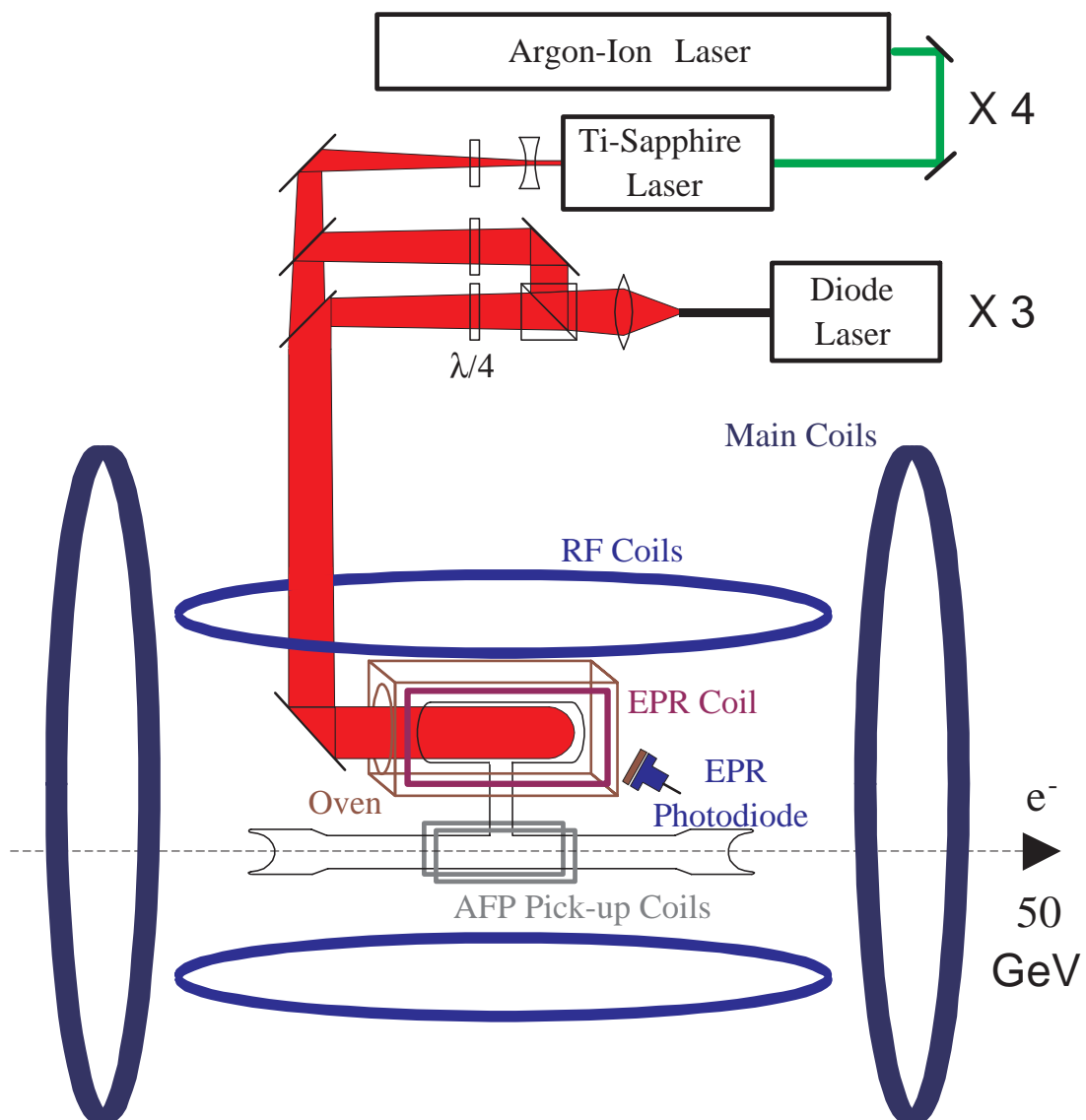
Fig. 5. The schematic of the E154 polarized target setup.
