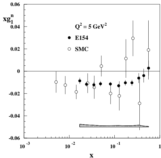
Fig. 8. A comparison of the E154 (closed circles) and SMC (open circles) data. The shaded area represents one standard deviation systematic errors.
