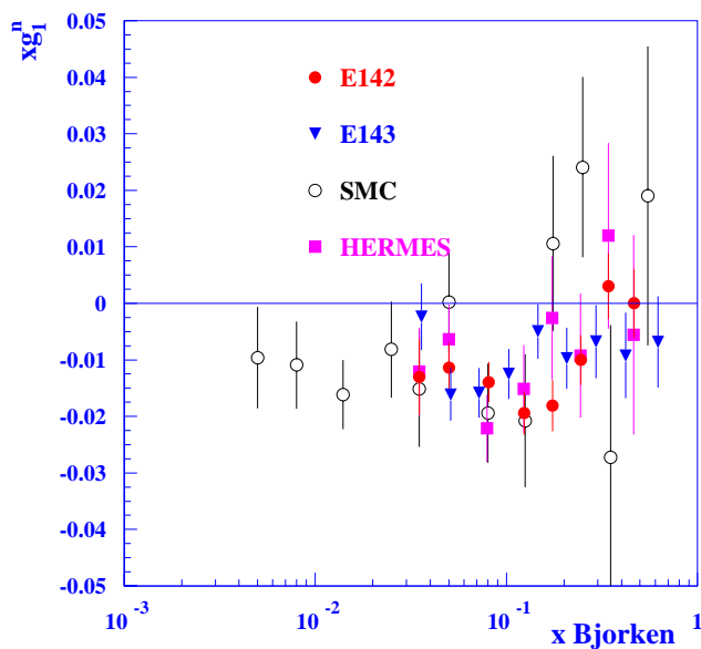
Fig. 3. World data on xg_1^n(x) .
