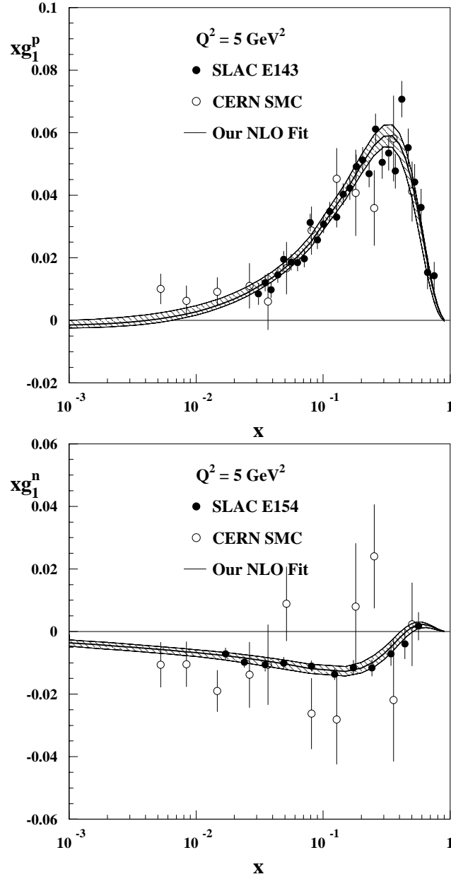
Fig. 12. The structure functions (top) xg_1^p and (bottom) xg_1^n at Q^2 = 5 \text{ GeV}^2 . E143, SMC, and E154 data have been evolved to Q^2 = 5 \text{ GeV}^2 using a procedure described in the text. The result of the \overline{\text{MS}} fit is shown by the solid line and the hatched area represents the total error of the fit.
