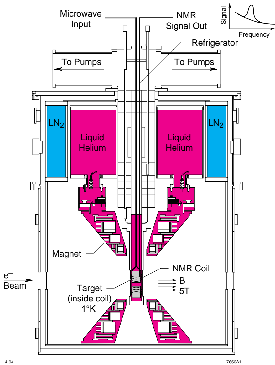
Fig. 6. The schematic of the E155 polarized target setup.
