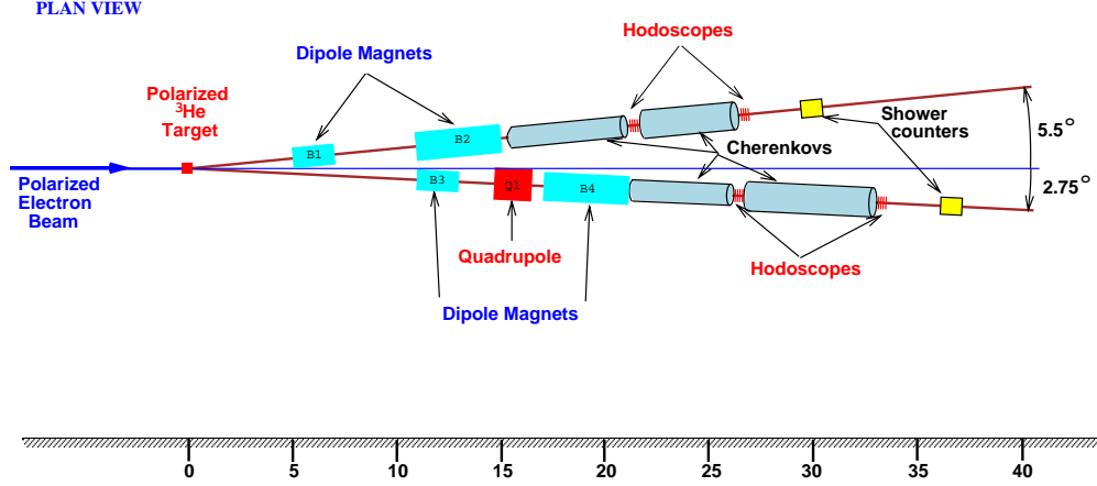
Fig. 7. Schematic plan of the E154/E155 spectrometers.
