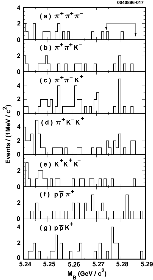
FIG. 1. Mass distributions for (a) B^+ \rightarrow \pi^+ \pi^+ \pi^- , (b) \pi^+ \pi^+ K^- , (c) \pi^+ \pi^- K^+ , (d) \pi^+ K^- K^+ , (e) K^+ K^+ K^- , (f) p \bar{p} \pi^+ and (g) p \bar{p} K^+ candidates. The signal region is between the arrows.
