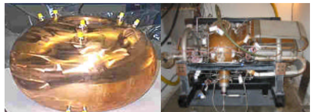
Figure 5: RF cavity body plated with leaky "brightened" copper (left) and leak-tight pure copper (right).
