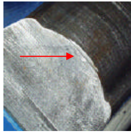
Figure 3: Sub-mm cut in quad chamfer reduced n = 6 multipole to <5 \times 10^{-4}</math>.
