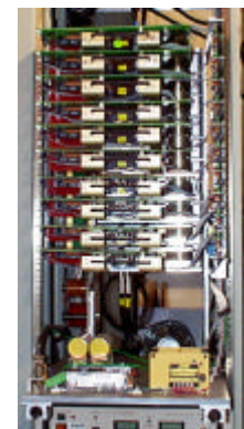
Figure 6: 15-kV IGBT kicker pulser.
