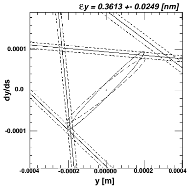
Fig. 6 Emittance plot in phase space and beam size
