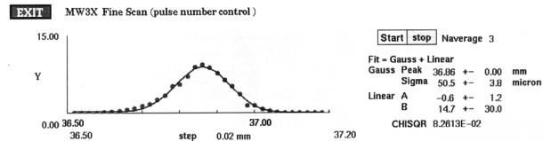
Fig. 4 Typical wire scan in Y
