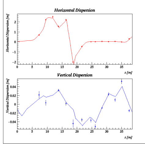
Fig. 3 Measured horizontal and vertical dispersion in the extraction line (plot) and fitted result (line).
