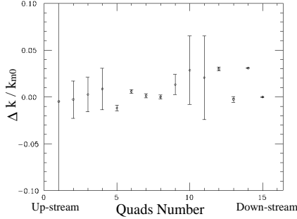
Fig. 2 Fitted relative errors of quads k-values
