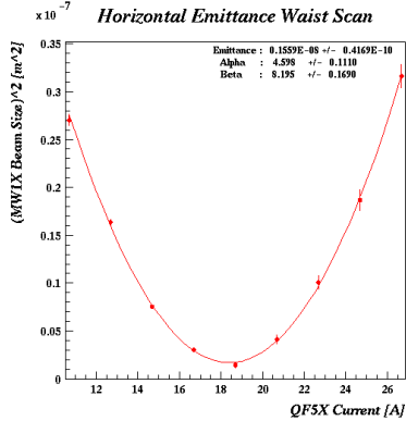
Fig. 5 Waist scan plot in X using QF5X
