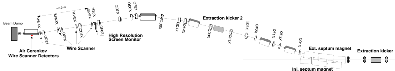
Fig. 1 Layout of the ATF-DR extraction line
