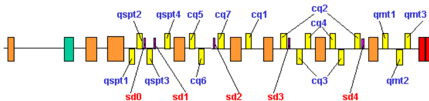
Figure 14.4 Quadrupole and Sextupole Families.
