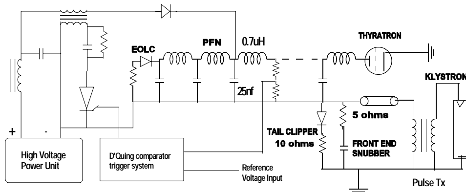
Figure 11.2 LIL klystron-modulator block diagram
