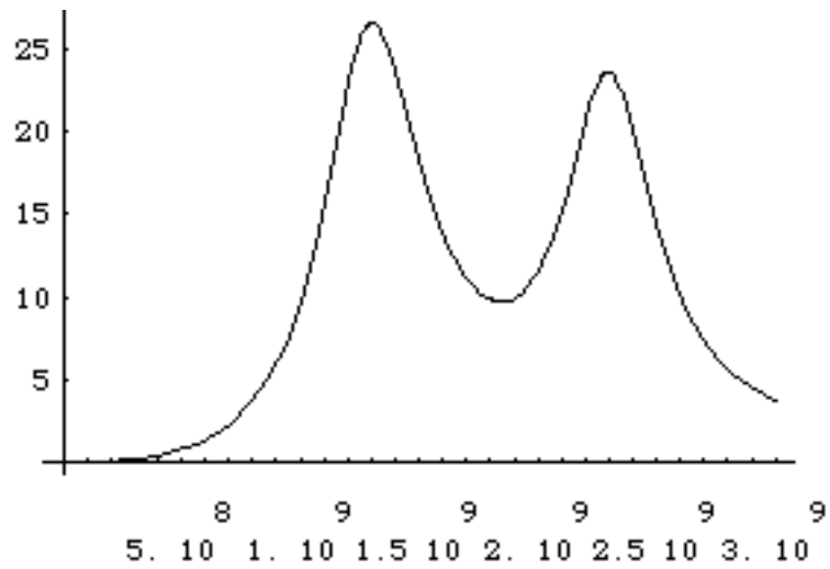
Figure 13.8 Real part of the BPM impedance.
