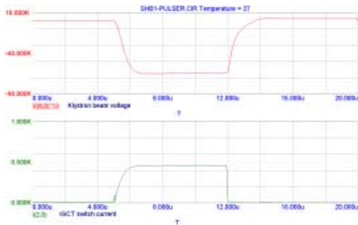
Figure 11.8 Simulation waveforms of SHB klystron-modulator
