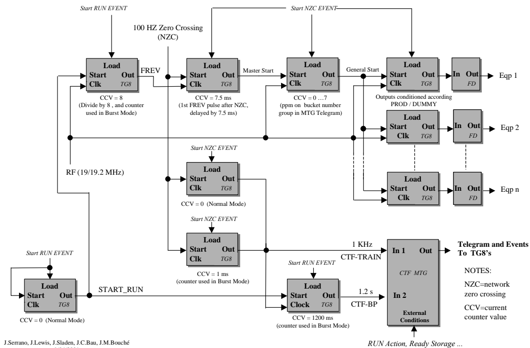
Figure 22.2.: Proposal for central timing for CTF3.
