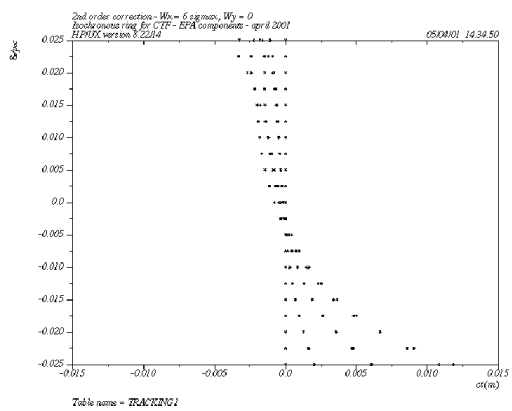
Figure 15.12 Path length with energy deviation and horizontal phase plane for sextupoles on.
