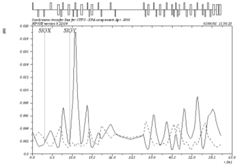
Figure 16.6 Transfer Lines Beam Envelopes (rms values)
