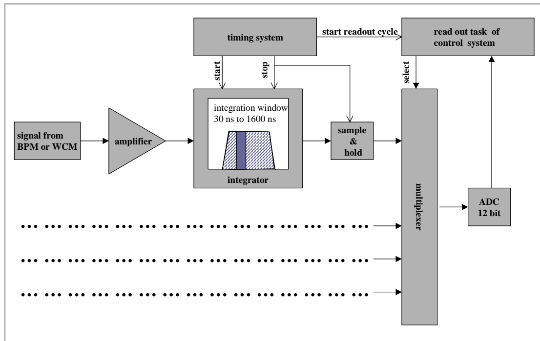
Figure 19.2 Data acquisition for BPM and WCM signals
