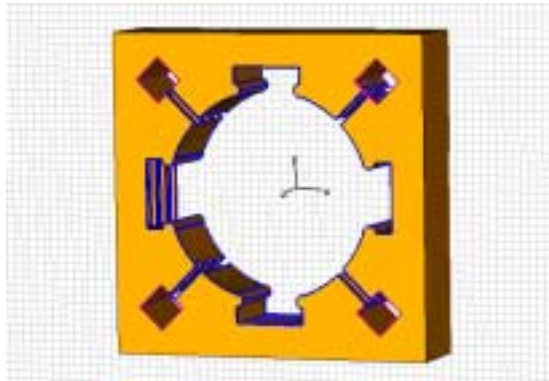
Figure 21.2 Waveguide PETS, 3 cells simulation
