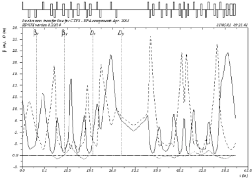
Figure 16.2 Transfer Lines Optical Functions
