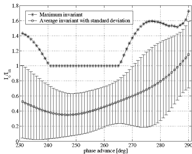
Figure 17.8 Tune dependence of the Courant-Snyder invariant magnification for an injection offset of 1 mm
