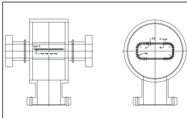
Figure 24.2 Typical pumping port with RF shield.
