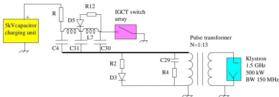
Figure 11.7 Basic SHB klystron-modulator circuit
