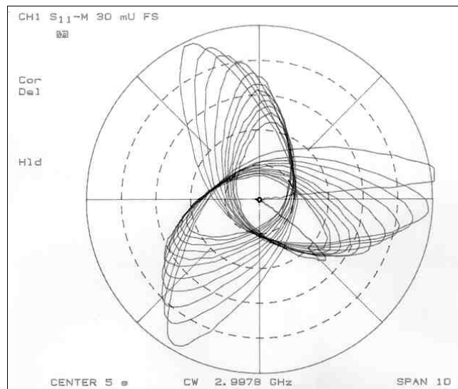
Figure 9.4 Bead-pull measurement: an error of about 40 ° between the 1 st and last cell is measured in this reflection diagram, corresponding to a phase slip of ±10 ° between electron and wave over 32 cells. The loss in accelerating efficiency is less than 1 %. The cells are not equipped with dimple tuners.
