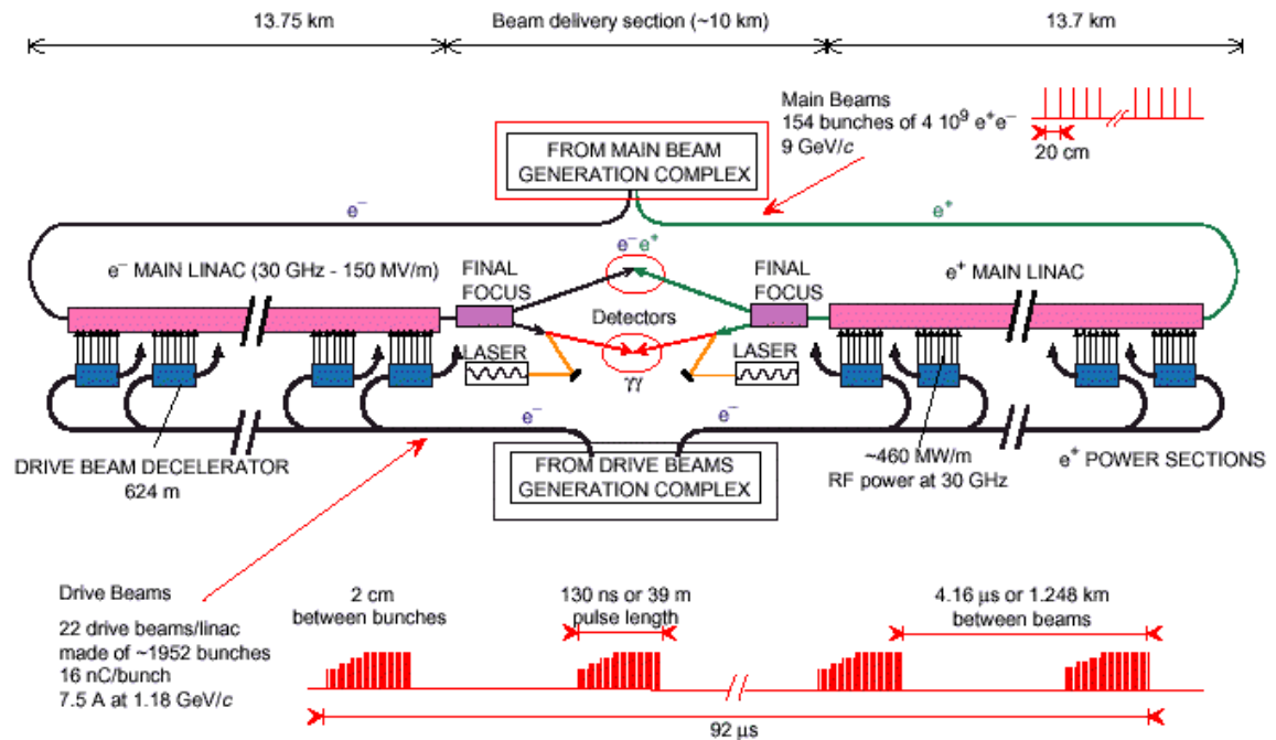
Figure 2.1 Generic Layout of CLIC
