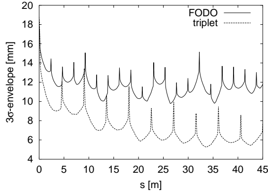
Figure 10.11 The 3- \sigma envelope of a beam that was injected with an initial offset of \Delta x = \sigma_x and \Delta y = \sigma_y
