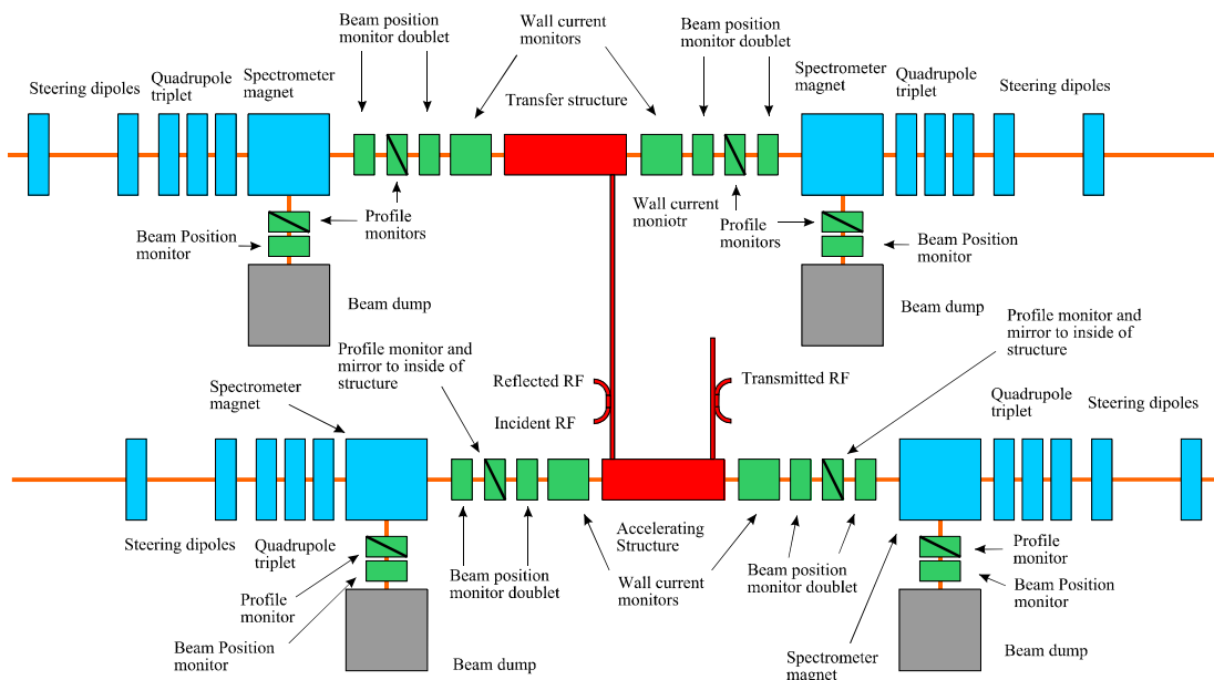
Figure 21.1.: Layout of Main Test Stand
