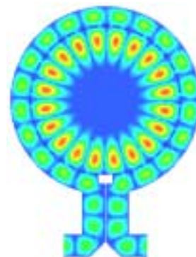
Figure 11.21 . Electric field plot in the BOC median plane.
