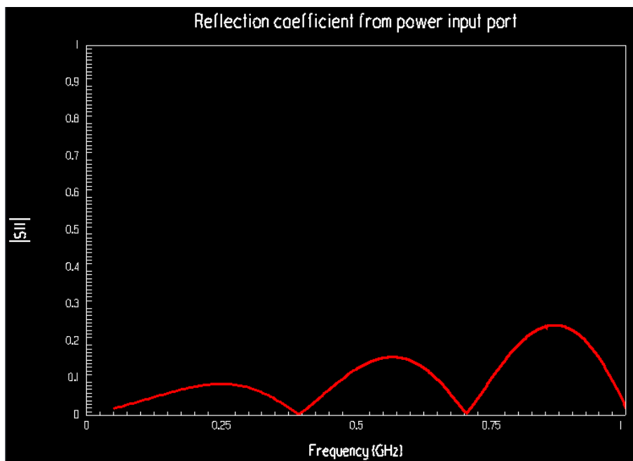
Figure 18.4 Reflection frequency response at the input ports (driven in the differential mode).
