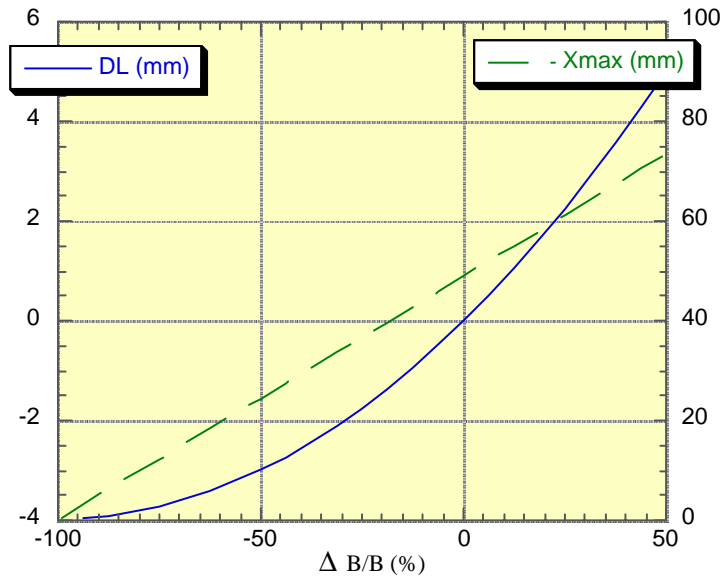
Figure 15.4 Path length variation (full line) as a function of wiggler field and maximum transverse displacement of the trajectory (dashed line).
