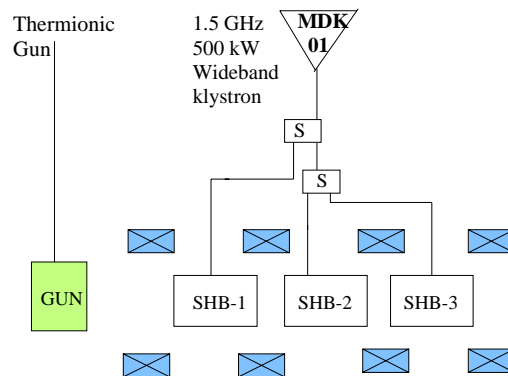
Figure 11.5 Klystron-modulator scheme for the SHB cavities
