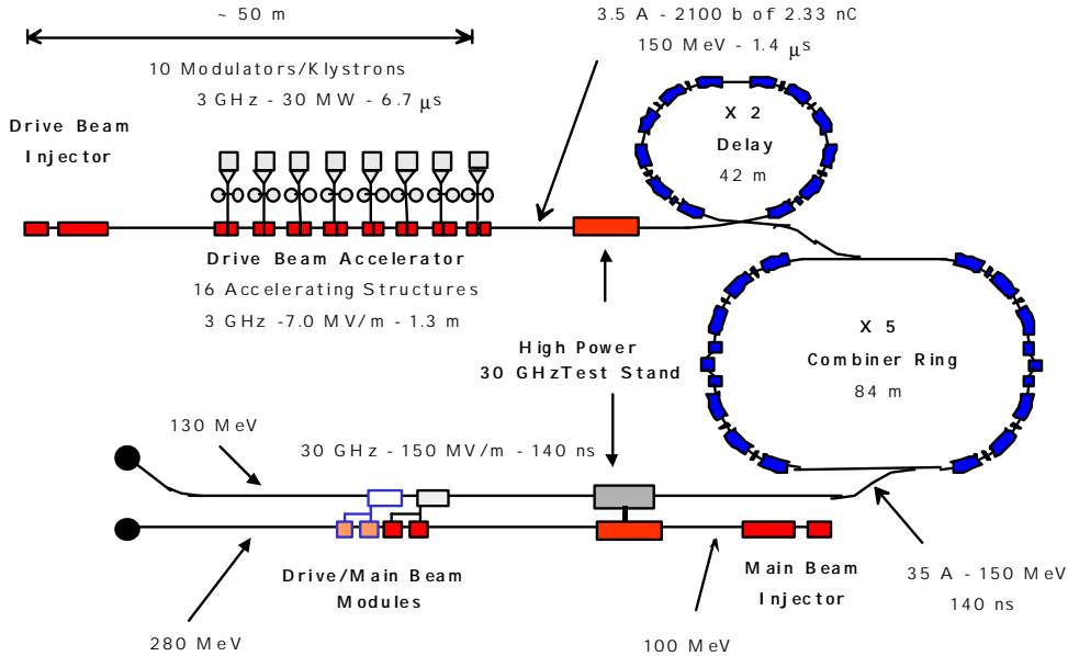
Figure 3.1 Conceptual layout of CTF3
