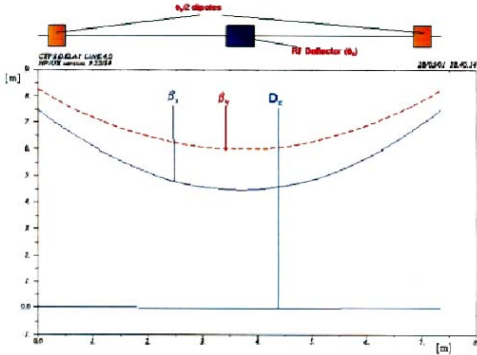
Figure 14.7 Even Bunches Line Optical Functions.
