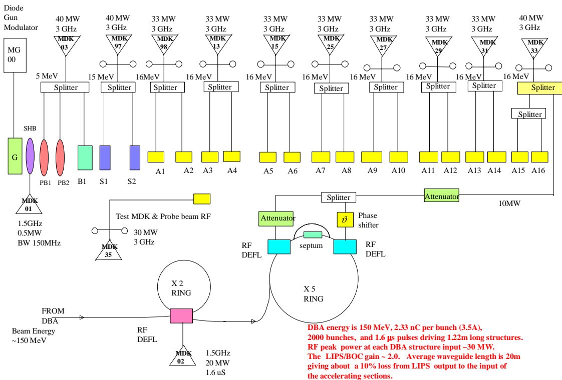
Figure 11.1 Basic klystron-modulator layout
