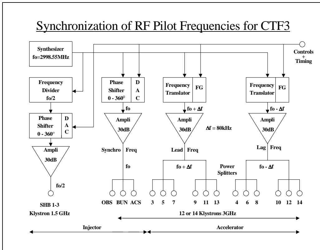
Figure 12.1 Block diagram of the RF distribution system.
