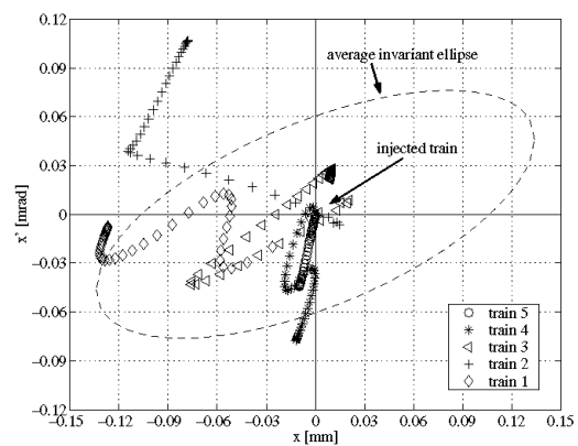
Figure 17.5 Phase space footprint of the bunch centres-of-mass of the merged trains
