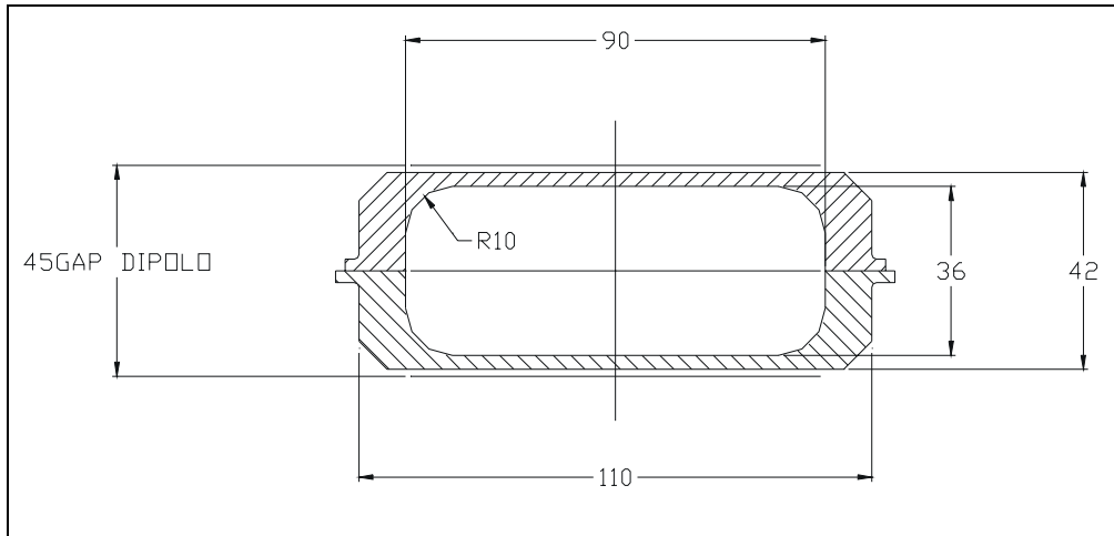
Figure 24.1 Typical cross section of the vacuum chamber, dimensions in mm.
