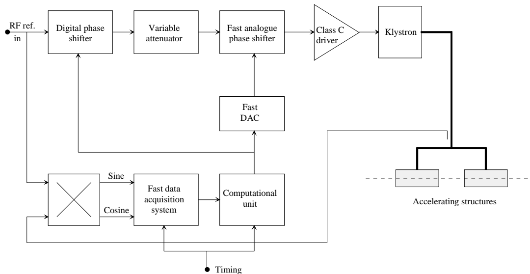
Figure 12.2 Block diagram of the phase control system
