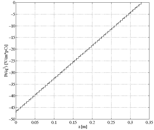
Figure 17.2 Multi-bunch wakes
