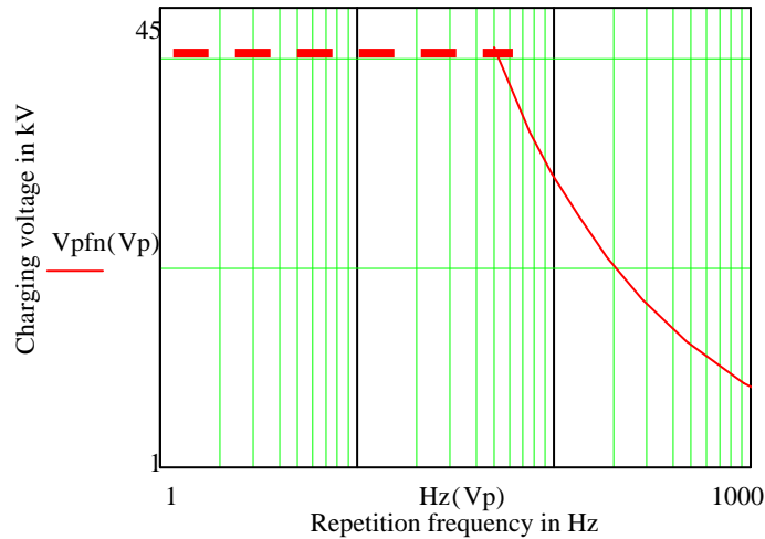
Figure 11.3 Charging voltage versus repetition frequency
