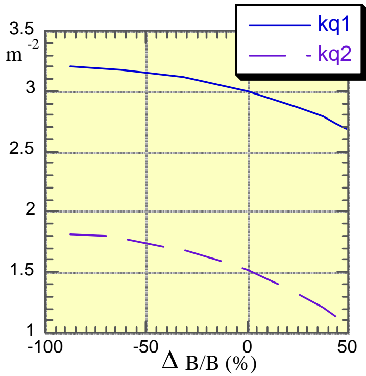
Figure 15.5 Strength of the wiggler section quadrupoles which match transverse betatron waists at the wiggler centre as a function of wiggler field.
