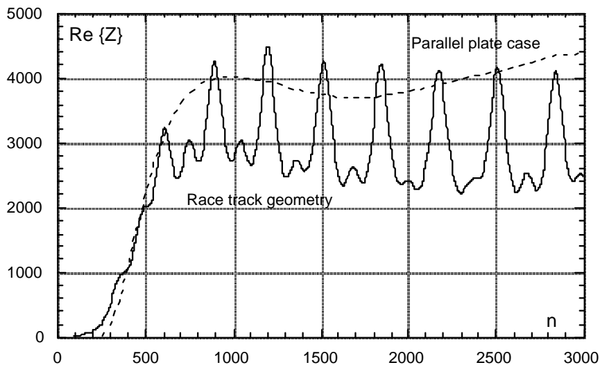
Figure 13.1 Real part of the CSR impedance
