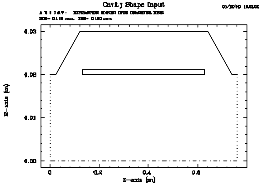
Figure 13.6 ABCI extraction kicker 2D model.
