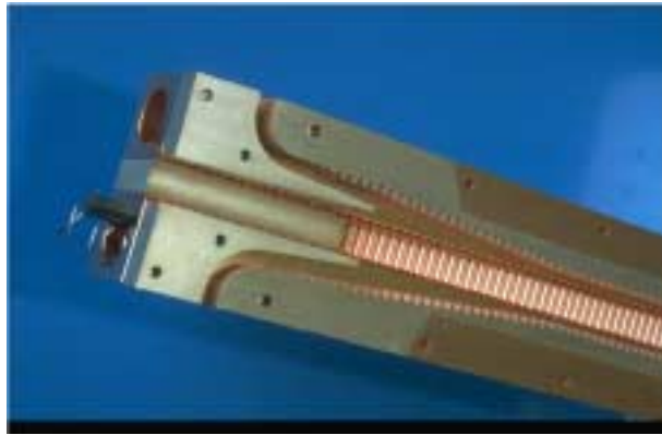
Figure 21.3 Open section of 15 mm aperture PETS
