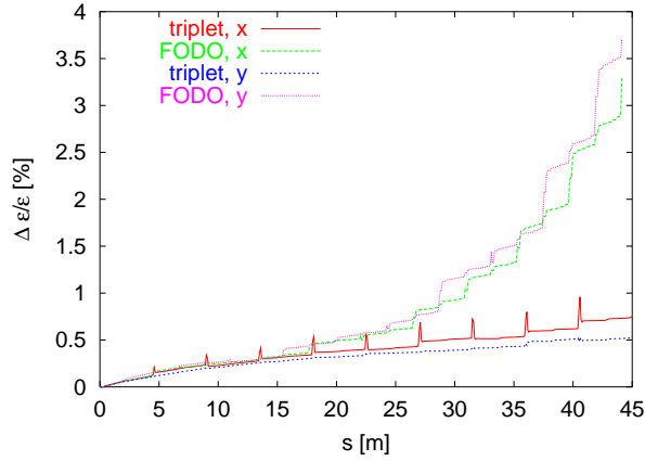
Figure 10.17 The emittance growth along the linac for the FODO and the triplet lattice.
