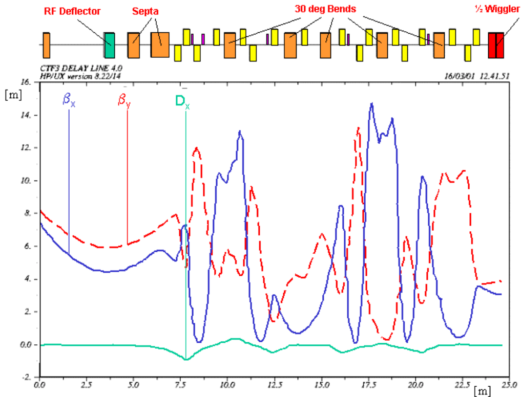
Figure 14.3 Delay Loop Optical Functions. Half Loop.
