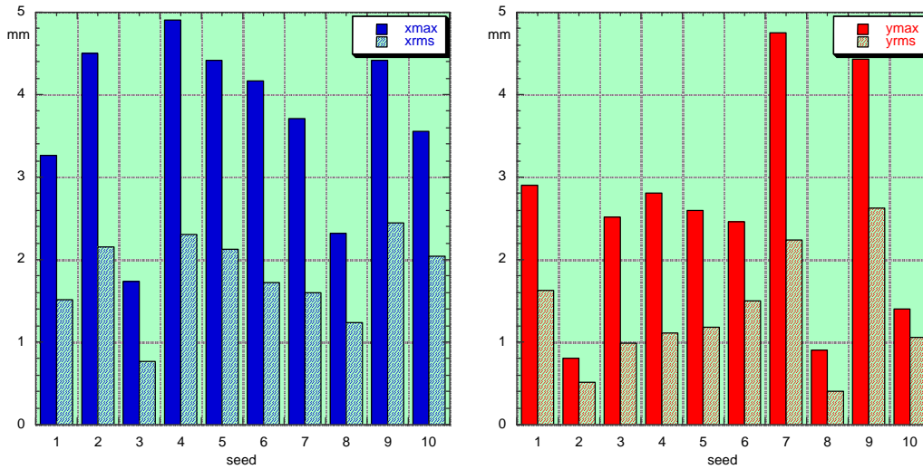
Figure 15.14 Closed orbit (horizontal and vertical) before correction
