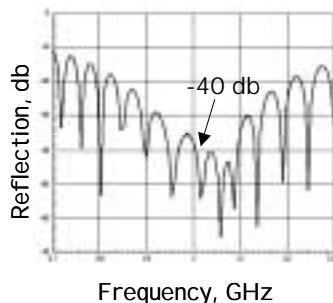
Figure 11.20 Matching of the waveguides
