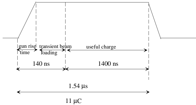
Figure 7.4 Pulse at the CTF3 gun exit
