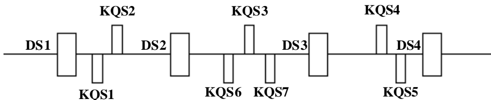
Figure 16.3 Four-bend achromat schematic layout
