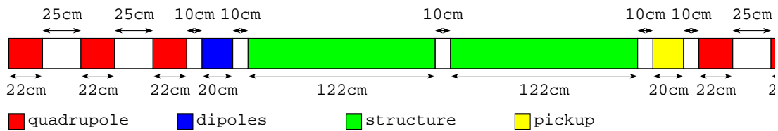
Figure 10.2 Sketch of a single cell in the triplet lattice.
