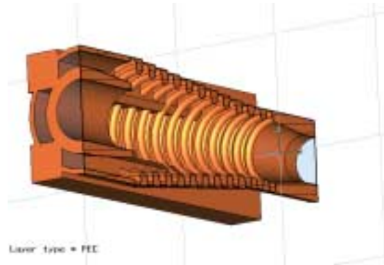
Figure 21.4 Cylindrical PETS output coupler simulation
