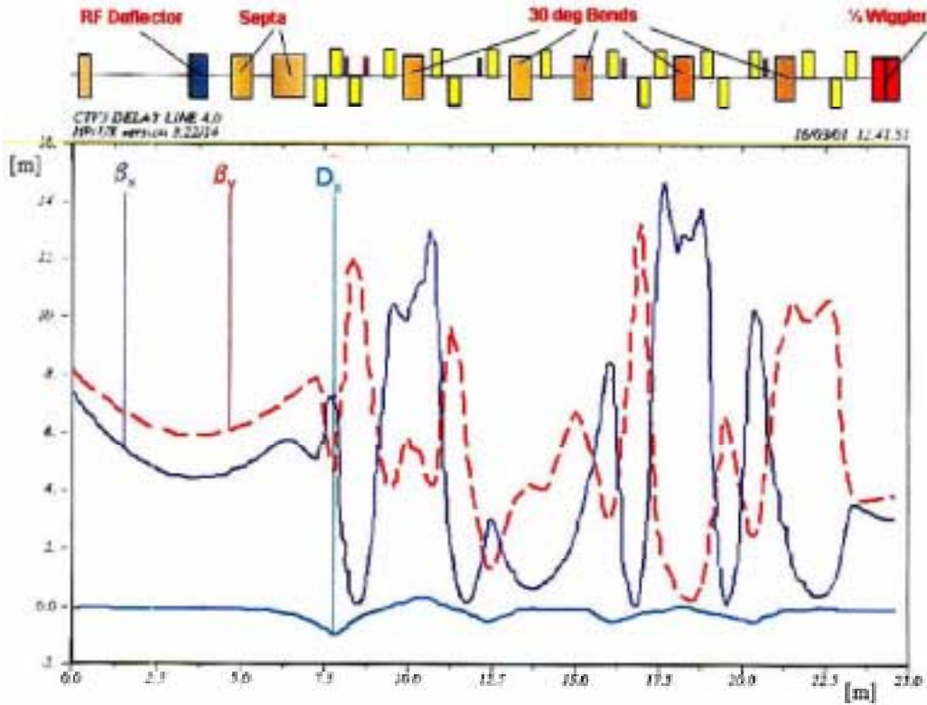
Figure 14.8 Delay Loop Beam Envelopes (rms values).
