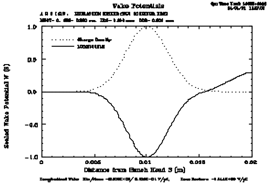
Figure 13.7 Extraction kicker wake potential of 2 mm bunch
