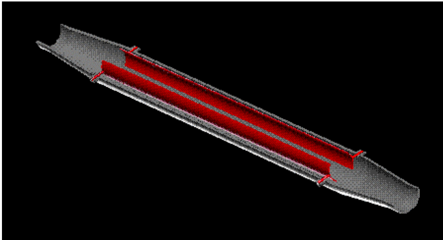
Figure 18.1 Extraction kicker inner structure
