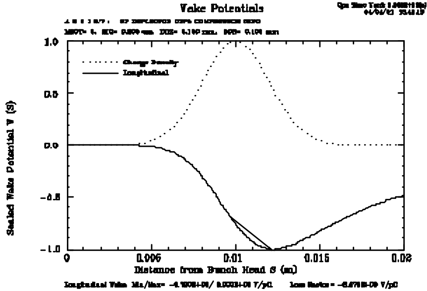
Figure 13.5 Wake potential of a 2 mm bunch in the RF deflector.
