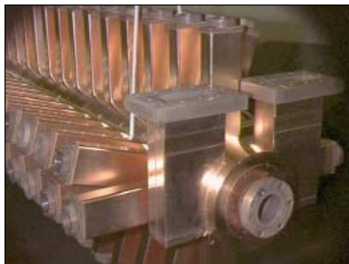
Figure 9.3 Brazed TDS ready for power testing
