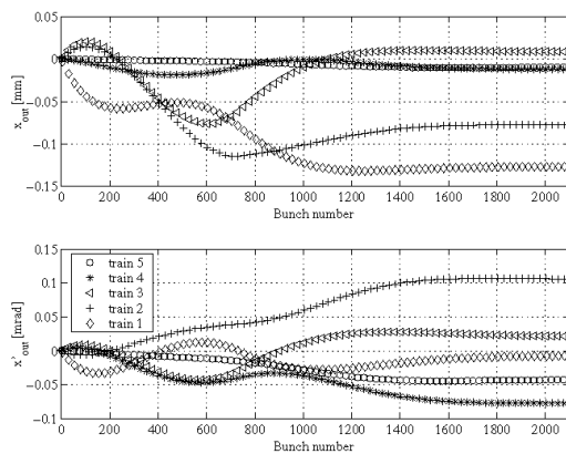
Figure 17.4 Position and angle of the bunches of the merged trains
