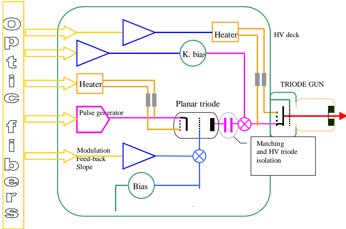
Figure 7.5 Schematic of the electronics for the gun.
