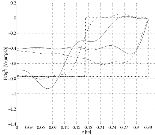
Figure 17.1 Single passage wakes
