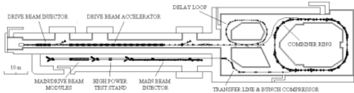
Figure 4.1 Implementation of CTF3 in the existing LPI building.
