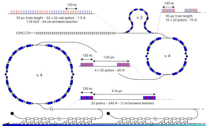
Figure 2.2 Drive beam structure of CLIC
