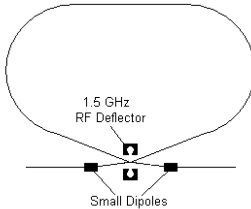
Figure 14.1 Delay Loop Injection Scheme.
