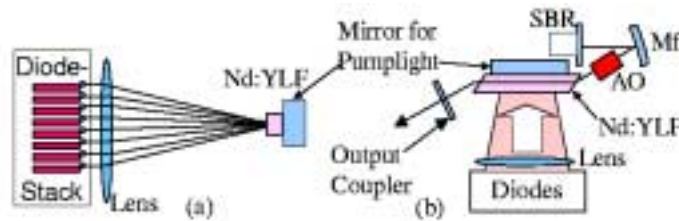
Figure 8.2 Schematic overview of the laser oscillator set-up. (a) Side view of the pump geometry. (b) Top view of the oscillator (Mf - curved folding mirror, AO - acousto-optic modulator).
