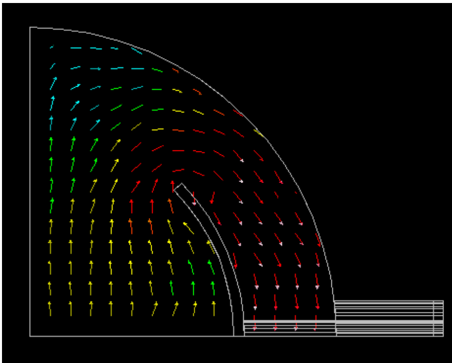
Figure 18.3 B-field distribution on a middle transverse plane in case of differential mode excitation.
