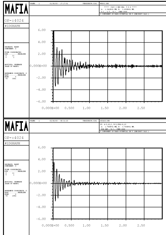
Figure 9.2 MAFIA time domain simulation of the dipole wake in the 32 nd cell of TDS (top) and SICA structure (bottom). Abscissa in m behind bunch centre, ordinate in V/(2 \text{ pC})/m/mm . Note the smaller short-range wake field in the SICA.
