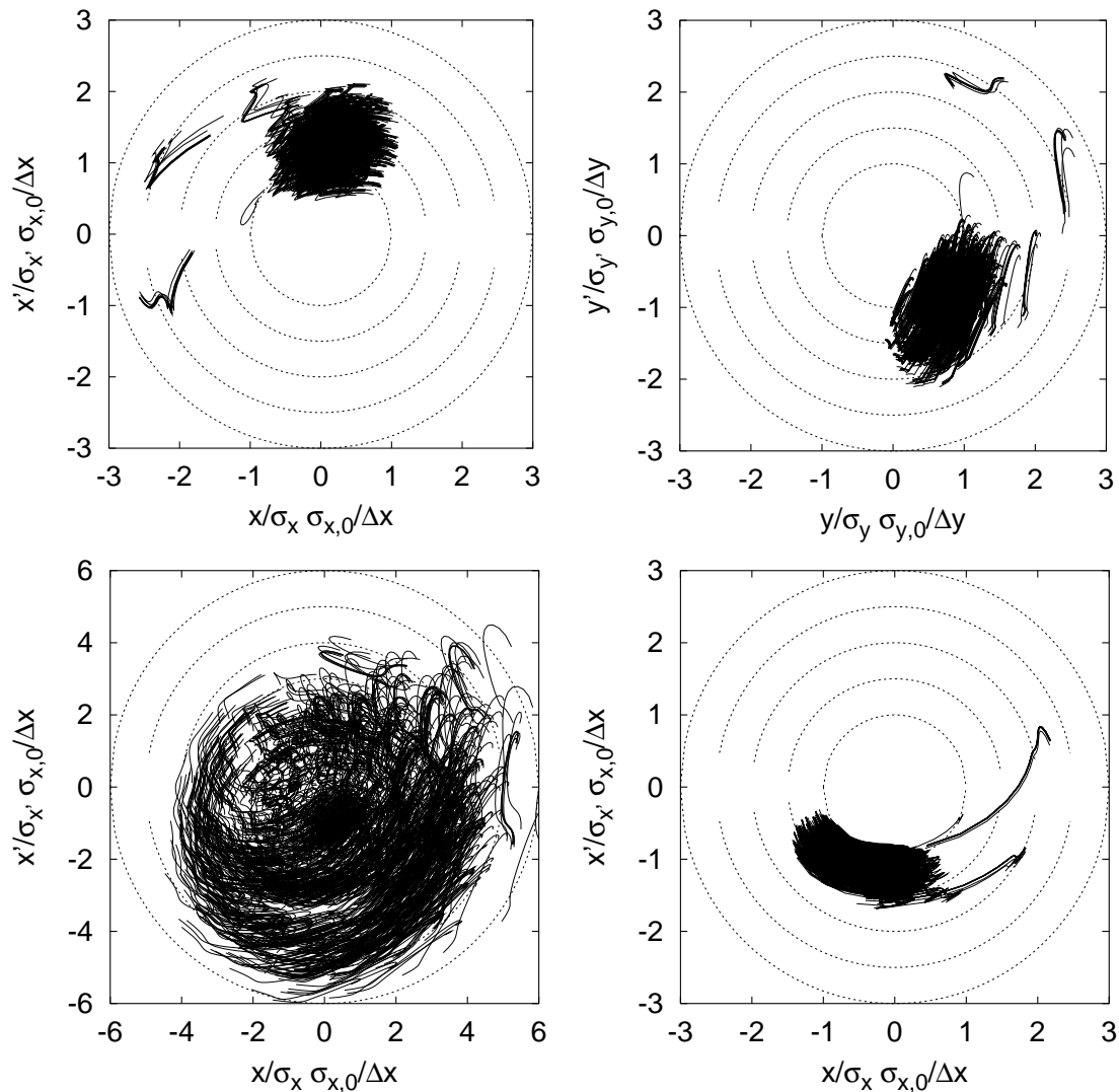
Figure 10.8 The final position of a beam with initial offset. The upper two plots show the horizontal and vertical plane in the triplet lattice. A few bunches at the intersection from one train to the next have significantly larger amplitudes than the rest of the beam. The third plot shows the beam at the end of the FODO lattice in the horizontal plane. The overall beam size has substantially increased. The last plot shows the jitter effect for a beam in the strongest triplet lattice (set number 0).
