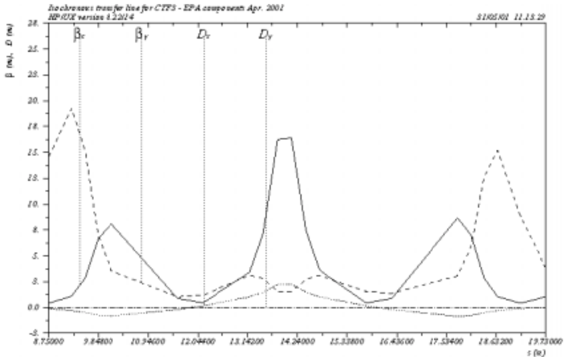
Figure 16.4 Four Bends Achromat Optical Functions
