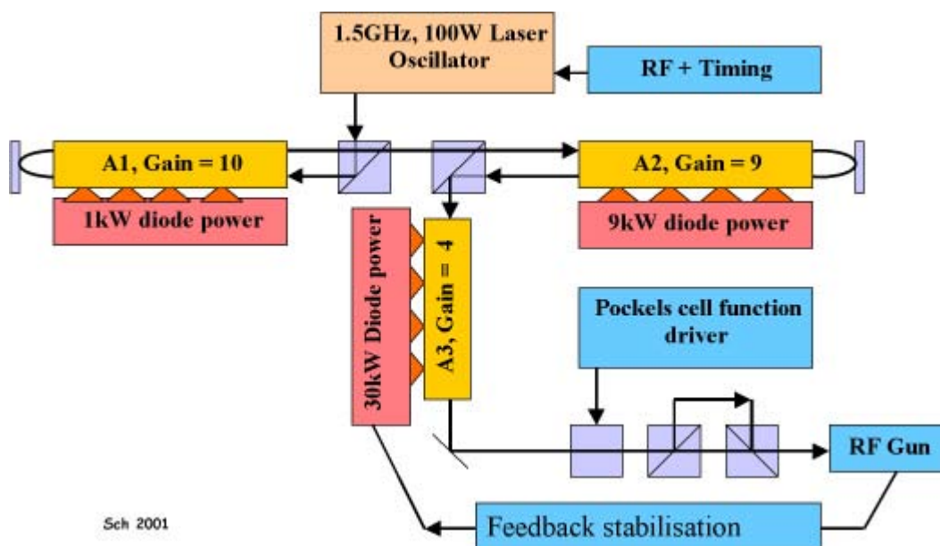
Figure 8.3 CTF3 Laser system
