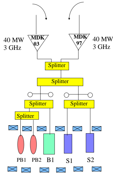
Figure 11.4 Dual klystron drive scheme for CTF3 injectors
