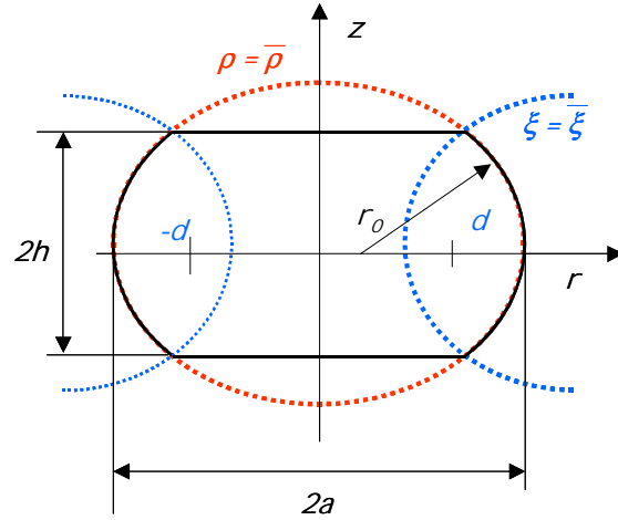
Figure 11.18 BOC profile
