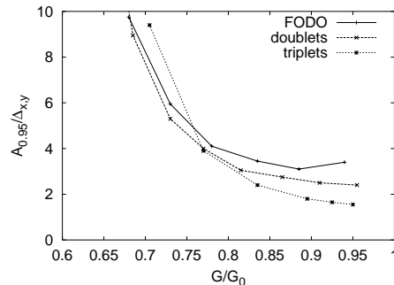
Figure 10.10 The amplification factor A_{0.95} versus the gradient error accepted in the lattices for the SICA.
