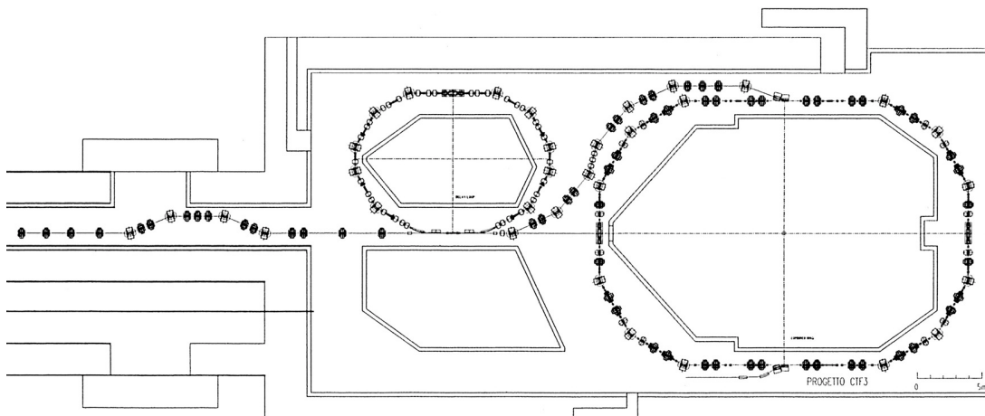
Figure 16.1 CTF3 Layout
