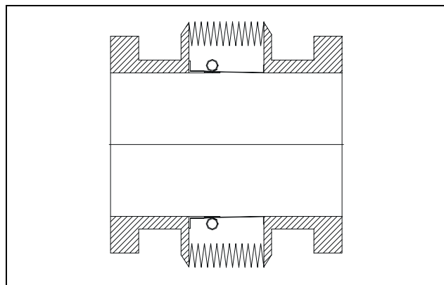
Figure 24.4 RF screened bellows.
