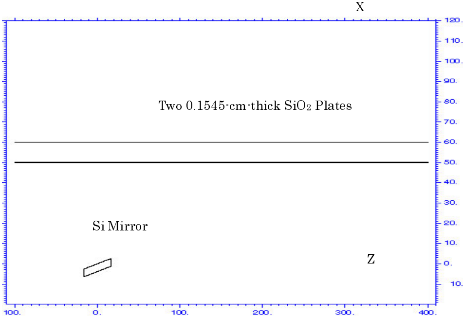
Fig 1. Geometry for the simulation of synchrotron radiation, emitted from the SPEAR3 bending magnet, hitting the Si mirror. The mirror is 9 degrees inclined relative to the beam direction (i.e., +Z axis). Polarization vector points toward +X. The shielding is two \text{SiO}_2 plates, parallel to the Z axis and each 0.1545 cm thick. The dose is scored at 1 m away from Z axis (i.e., X=100 cm).
