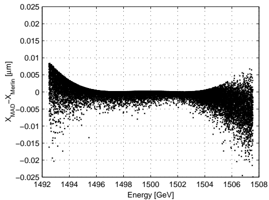
Figure 2: Difference of the horizontal particle position at the end of the BDS versus particle energy, as calculated by Mer1.in and MAD.
