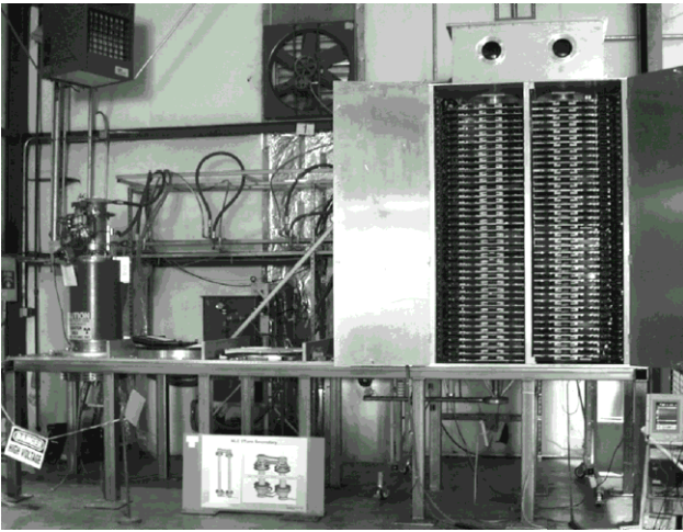
Figure 6. Assembled stack
