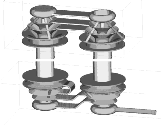
Figure 7. Three turn design
