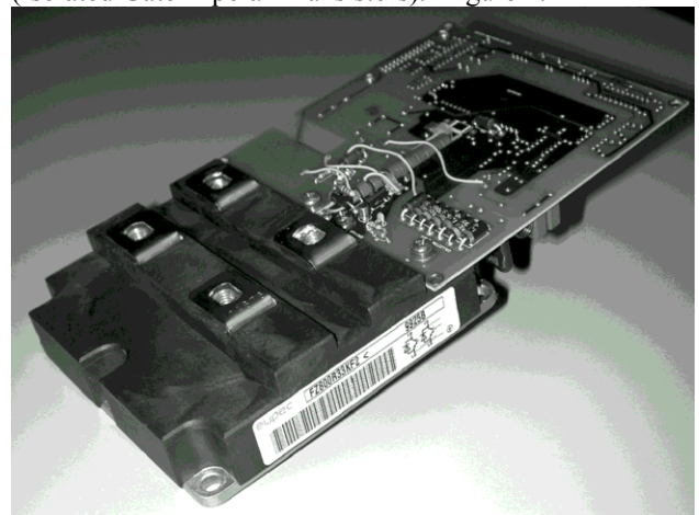
Figure 2. IGBT & Gate Driver
