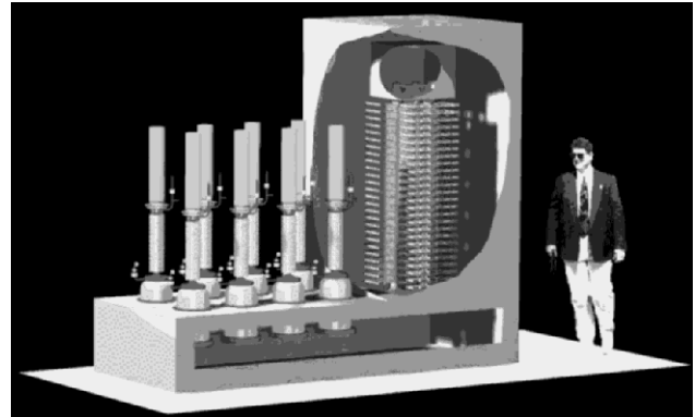
Figure 1. Induction Modulator Artistic Rendition
