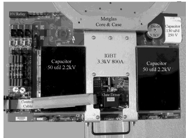
Figure 4. IGBT Drives boards
