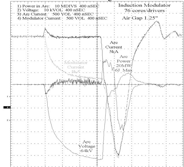
Figure 9. Arc over tests in air
