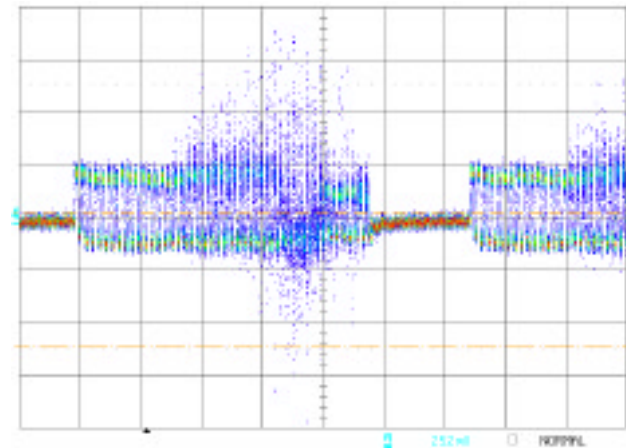
Figure 3: E+ correction signal with 45/60 bunches ( \sim 400\text{mA} )
