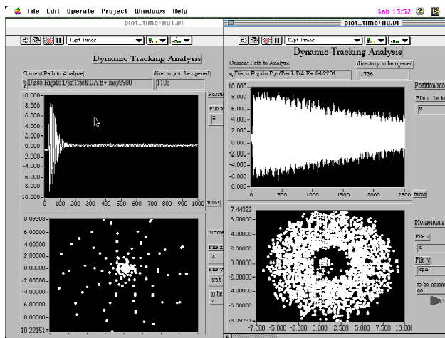
Figure 3: Dynamic tracking measurements of the beam transverse displacement vs number of turns (above), and phase space trajectory (below). The case with wiggler on is shown on the left, wiggler off on the right.
