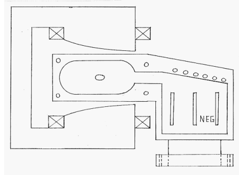
Figure 1 Possible magnet and vacuum chamber for the HER of a SBF.
