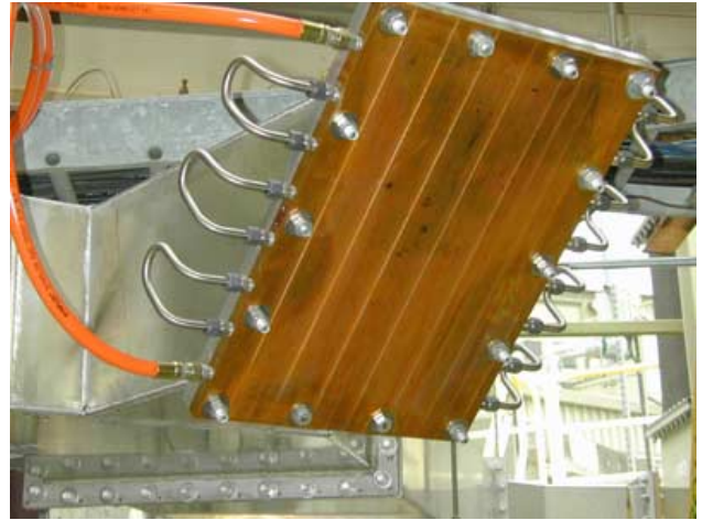
Figure 4: Finished waveguide load installed and in operation.
