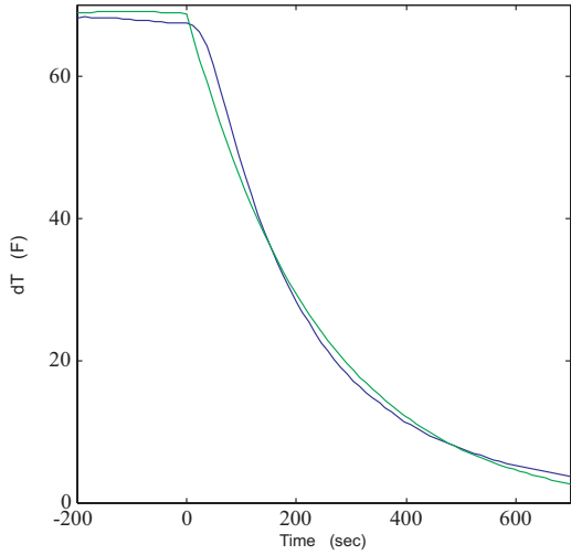
Figure 2: Response of thermocouple (blue) and exponential weighting from positron current (green) for a step change of -1.25 A.
