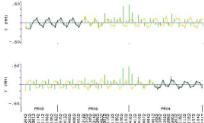
Figure 4: BPM data with xy -orbit fit.
