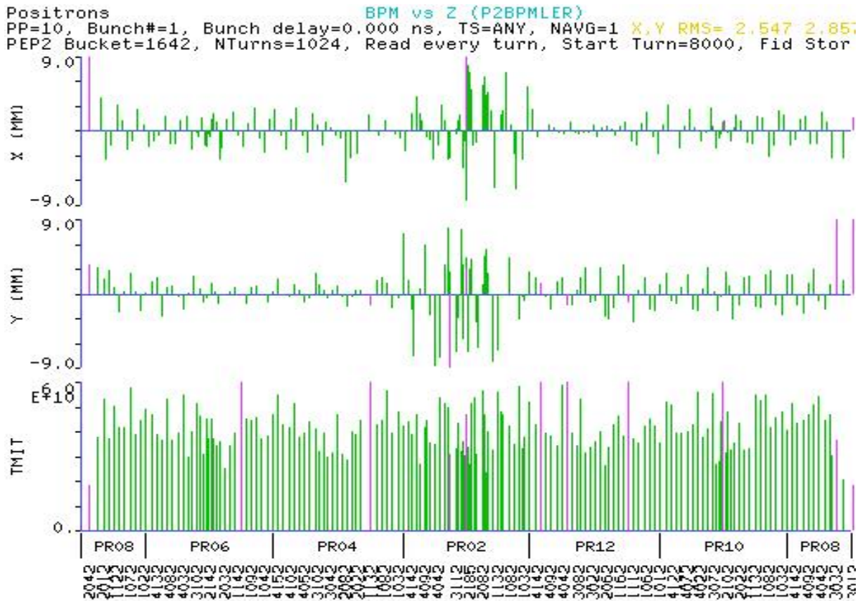
Figure 1: LER orbit showing the wild oscillation of 9 mm near the interaction point (PR02).
