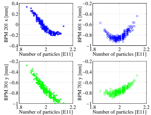
Fig. 6: Transverse jitter at the end of the linac. The jitter in x and y is strongly correlated with intensity and energy along the linac, because of beam loading. This dispersive jitter can be reduced from of 300 \mu\text{m} to 25 \mu\text{m} rms by launching oscillations early in the linac. A quadratic term is also visible here.
