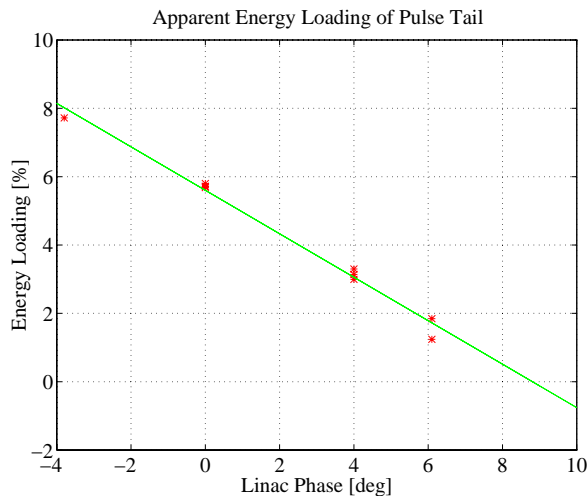
Fig. 5: Measured beam loading for different linac phases. Since the beam loading before the chicane is transformed into phase loading, the slope of the linac RF can be used to counteract the loading jitter in the main part of the linac. A +9^\circ linac phase off the crest would reduce the energy jitter totally, but the single bunch energy spread due to the bunch length becomes too large.
