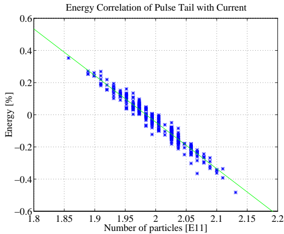
Fig. 4: Beam energy versus current. The beam loading of the high current beam reduces the energy of the tail of the bunch for higher charges: -0.58\% for a 10\% total charge variation, which is 5.8\% beam loading (for 100\% ). A higher intensity beam will have a lower energy and will follow a longer path through the chicane, arriving later. When the bunches ride earlier than the RF crest, the tail or later particles will go up the RF slope canceling the stronger beam loading due to the higher intensity. A rough estimate gave a phase offset of about 12^\circ for a perfect cancellation, which is close enough to give measurable results. The measurement (Fig. 5) shows an extrapolated perfect cancellation at 9^\circ , but the single beam energy spread due to the bunch length was too large to get the beam through the energy defining slits. Shorter bunches with an additional compression near the middle of the linac would make it possible to use this effect [2].
