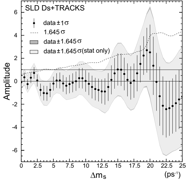
FIG. 2: Measured B_s^0 oscillation amplitude as a function of \Delta m_s . The light-grey (dark-grey) band shows the 90% confidence region obtained from statistical (total) uncertainties. Values of \Delta m_s for which the allowed band is below A = 1.0 are excluded at the one-sided 95% confidence level.
