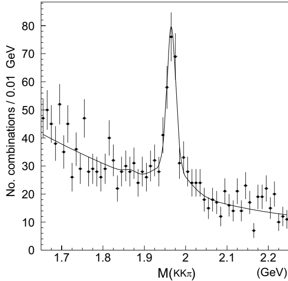
FIG. 1: Distribution of KK\pi invariant mass for \phi\pi and K^{*0}K candidates combined, for the events that include a B_s^0 candidate vertex. The solid line shows a fit with the same functional form as is used in the likelihood function: two Gaussian distributions with common mean for the D_s signal, a single Gaussian for the D^+ contribution and a second-order polynomial for the background.
