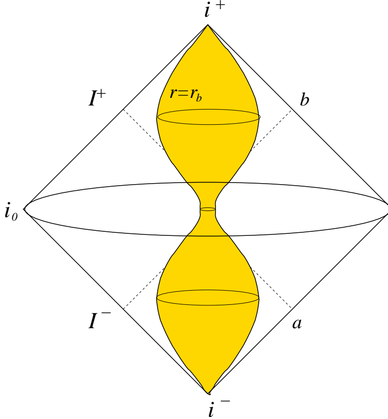
Fig. 4: Penrose diagram of the four dimensional Kerr bubble, with null rays a and b separating the “Milne” and “de Sitter” epochs.
