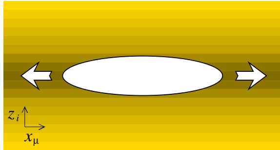
Fig. 5: Asymmetric expansion of a hybrid bubble. In the darker region, local supersymmetry is broken to a larger extent; local supersymmetry emerges asymptotically at large z . It seems that the space-eating bubbles do not find the regions of unbroken local supersymmetry very tasty.
