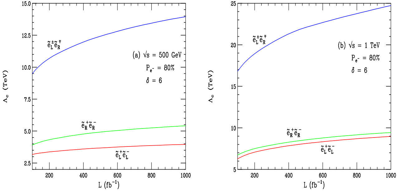
FIG. 3: 95% C.L. search reach for \Lambda_c in each production channel as a function of integrated luminosity for \sqrt{s} = 0.5 and 1.0 TeV.
