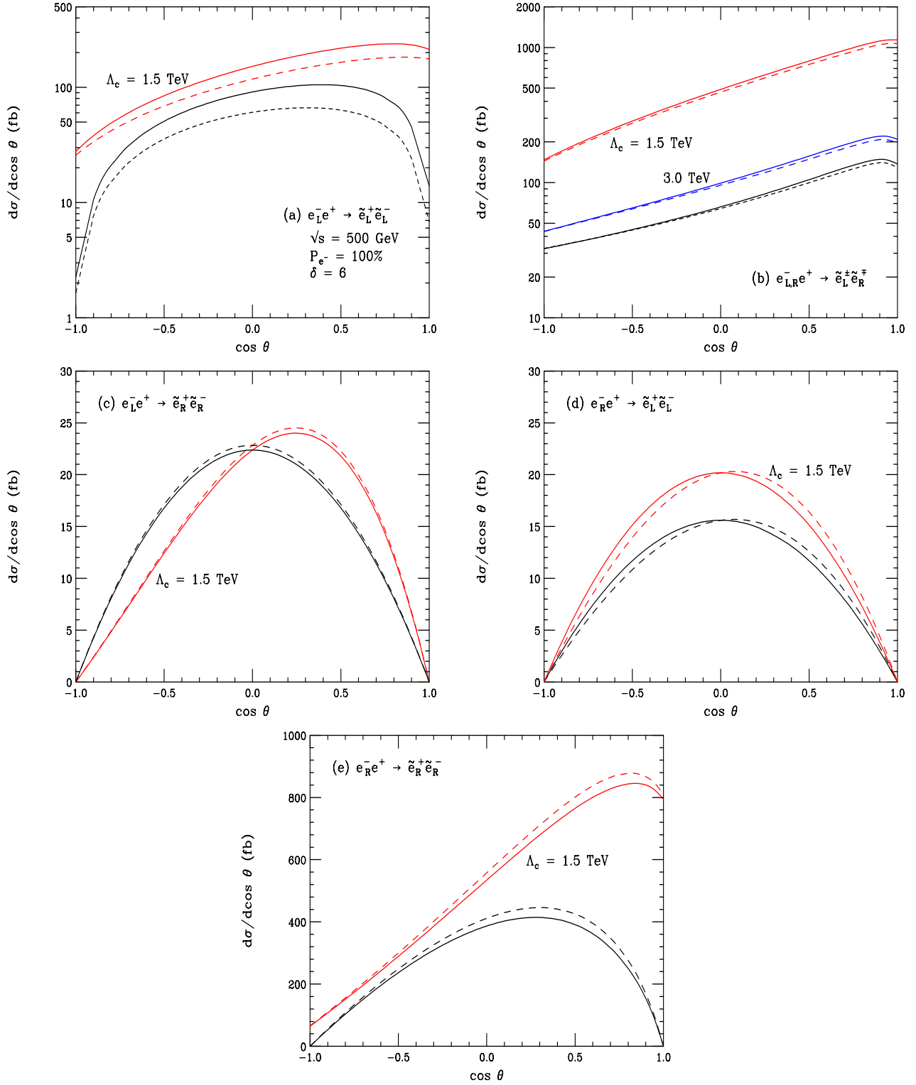
FIG. 1: Angular distributions for each helicity configuration with supersymmetric bulk contributions for \Lambda_c = 1.5 \text{ TeV} (top curves), and for the D = 4 supersymmetric models (bottom curves). The solid (dashed) curves correspond to a bino-like (Higgsino-like) composition of the lightest neutralino.
