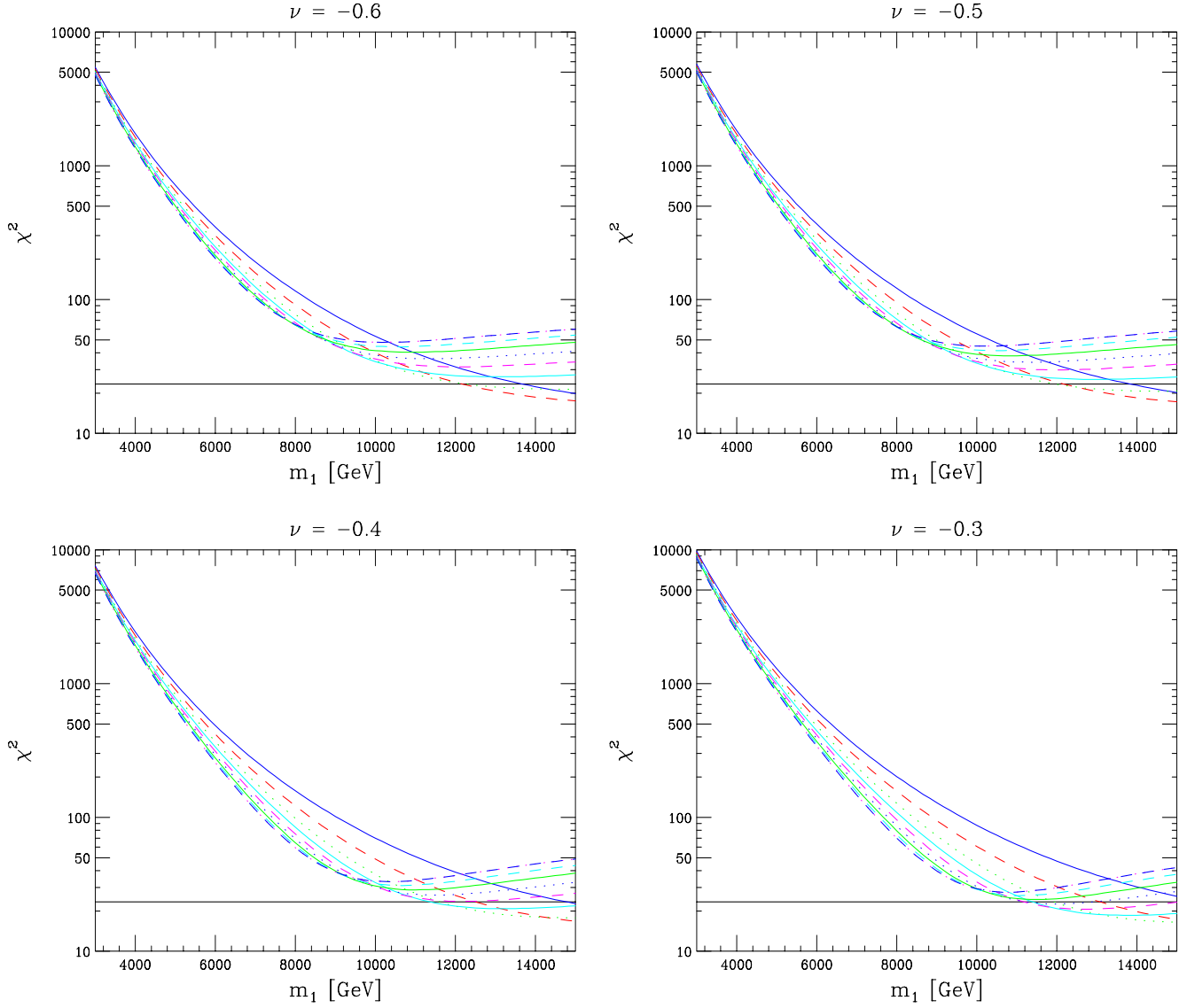
Figure 4: Plots of the \chi^2 values obtained in the fit to the EW precision data versus m_1 for four choices of \nu , the fermion bulk mass parameter. The solid black line indicates where \chi^2 = 23.3 , the value at which the 95% CL is reached. The colored curves are the RS model fit results for different Higgs boson masses; from top to bottom, on the left of each plot, the lines indicate m_H = 115, 200, 300, \dots, 1000 GeV.
