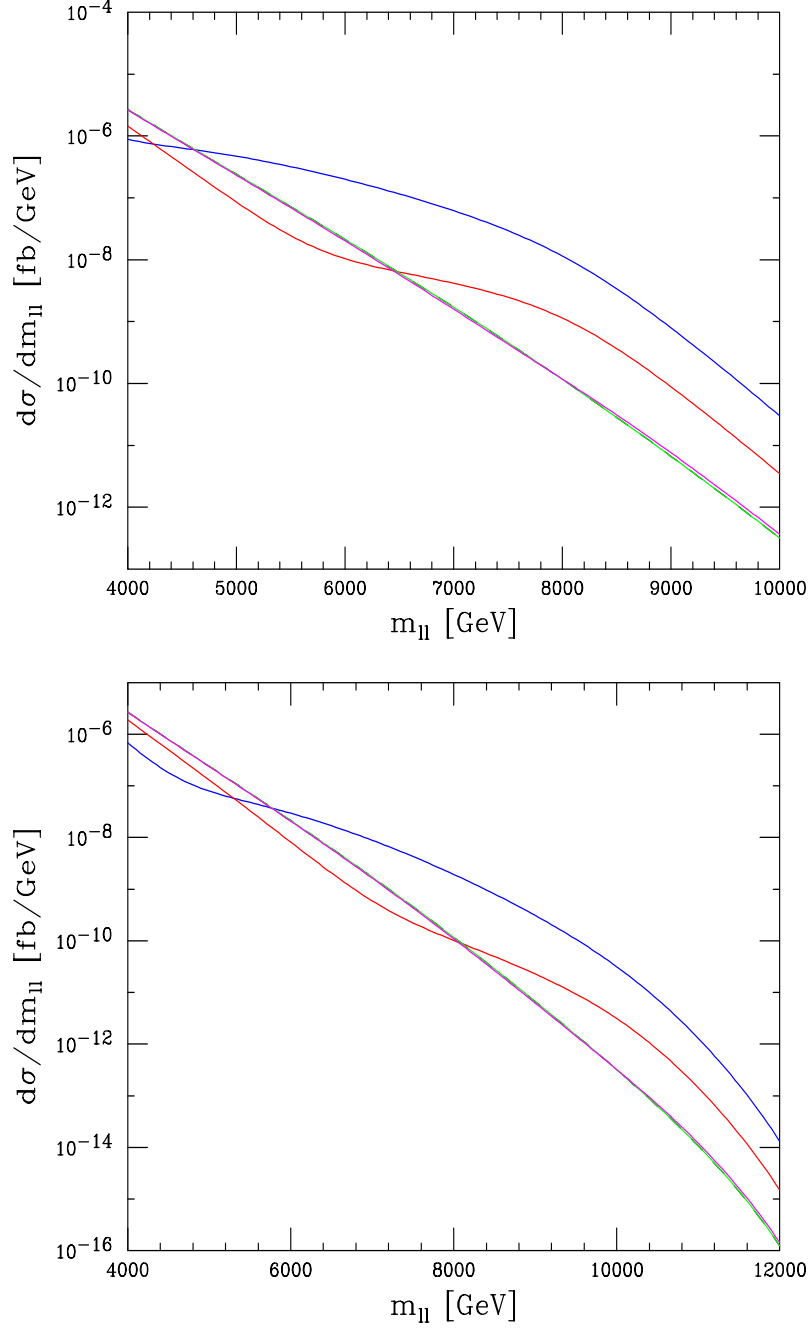
Figure 6: Cross sections for the process pp \rightarrow \mu^+\mu^- for m_1 = 8 TeV (top) and m_1 = 10 TeV (bottom) as functions of the final state lepton invariant mass. The upper blue curves are the results for \nu = -0.3 , the slightly lower red curves the cross sections for \nu = -0.4 , and the three nearly degenerate straight lines on each plot the results for \nu = -0.5, -0.6 , and the SM. K-factors and a rapidity cut |\eta| < 2.5 have been included.
