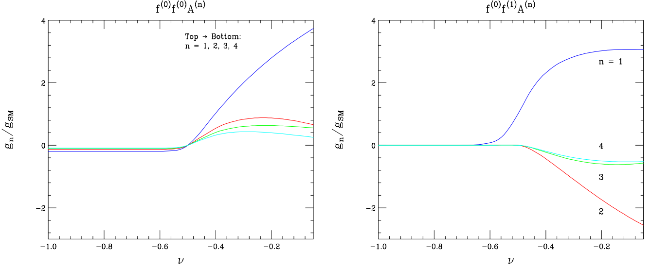
Figure 1: Plots of the coefficients C_{f\bar{f}A}^{00n} (left) and C_{f\bar{f}A}^{01n} (right) for n = 1, \dots, 4 as functions of the fermion bulk mass parameter \nu .
