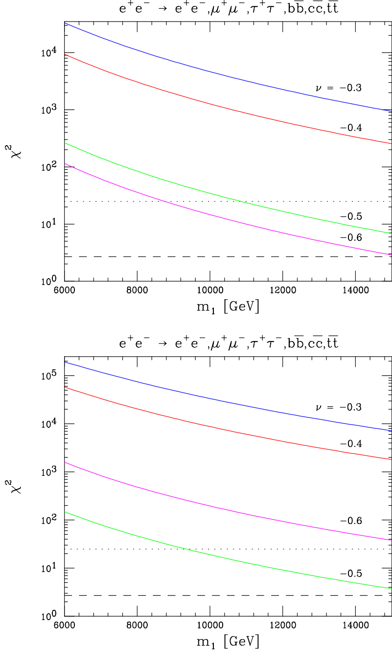
Figure 9: \chi^2 values obtained by fitting the RS model predictions for fermion pair production to the SM for \nu = -0.6, -0.5, -0.4, -0.3 , as functions of m_1 . The upper plot assumes \sqrt{s} = 500 GeV and L = 500 fb ^{-1} , while the lower assumes \sqrt{s} = 1000 GeV and L = 1000 fb ^{-1} . The solid straight line indicates the \chi^2 necessary for exclusion of the model at the 95% CL, and the dotted line illustrates the \chi^2 required for a 5 \sigma discovery. The polarizations and reconstruction efficiencies assumed are presented in the text.
