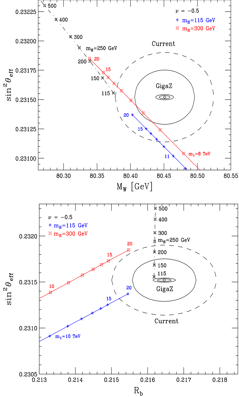
Figure 10: Plots of the \sin^2 \theta_{\text{eff}} versus M_W plane (top) and \sin^2 \theta_{\text{eff}} versus R_b plane (bottom) showing current and future sensitivities, SM predictions, and RS model predictions. The diamonds show the current measured values. The large solid and dashed ellipses represent respectively the 68% and 95% CL regions from current sensitivities, while the smaller solid ellipses anticipate the same after operation of GigaZ. The black dashdot lines show the SM predictions for different Higgs boson masses, while the three solid colored lines show the RS model results for varying m_1 and for two Higgs masses satisfying the current EW constraints.
