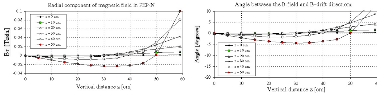
c) DV06b field map (the best design by the time of the workshop):
