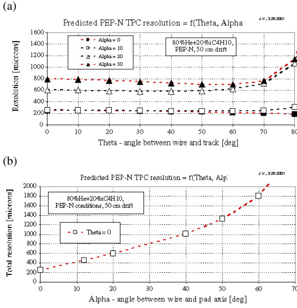
Figure 4: Predicted resolution per sample in the PEP-N TPC in a slow 80%He + 20% \text{C}_4\text{H}_{10} gas a function (a) \Theta and (b) \alpha angles, defined in Figure 3.
