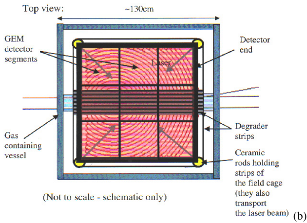
Figure 7: Field cage—top view. The picture also shows the radial pattern of the GEM readout strips ( \sim 3 cm long, \sim 5 cm wide), carbon strips along the beam line, field cage with ceramic rods and Mylar strips, and outer Hexel gas containing enclosure.
