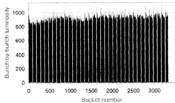
Figure 2. The measured luminosity in each bunch along the bunch train. Note that the luminosity dips where the LER RF phase has maxima.
