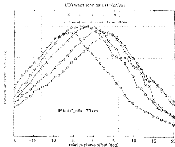
Figure 3. Variations in luminosity with HER RF phase as a function of location of the LER vertical beta waist.
