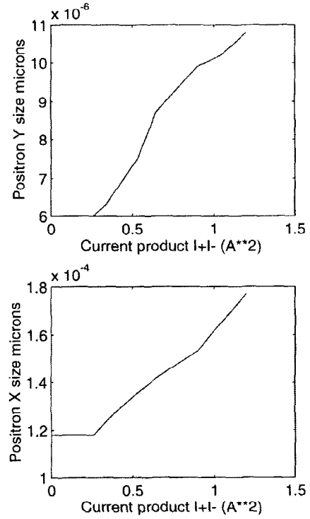
Figure 7. Measured LER positron beam sizes as a function of the product of the beam currents.
