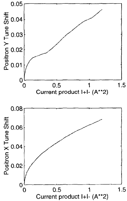
Figure 8. Derived beam-beam tune shift parameters versus current for LER positrons.
