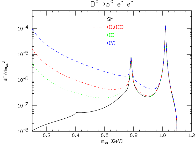
Figure 11: The dilepton mass distribution for D \rightarrow \rho^0 e^+ e^- (normalized to \Gamma_{D^0} ), in the MSSM with non-universal soft breaking effects. The solid line is the SM; (I): M_{\tilde{g}} = M_{\tilde{q}} = 250 GeV; (II): M_{\tilde{g}} = 2 M_{\tilde{q}} = 500 GeV; (III): M_{\tilde{g}} = M_{\tilde{q}} = 1000 GeV and (IV): M_{\tilde{g}} = (1/2) M_{\tilde{q}} = 250 GeV.
