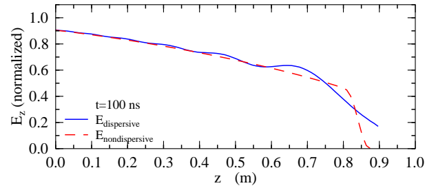
Figure 4 A snapshot E_z fields in the vg5 0.9-m structure: solid) dispersive on; dashed) dispersive off.
