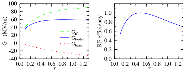
Figure 2 Gradient and efficiency as functions of \tau . The beam loading current is 0.9-amp. The RF power per unit structure length is 97-MW.
