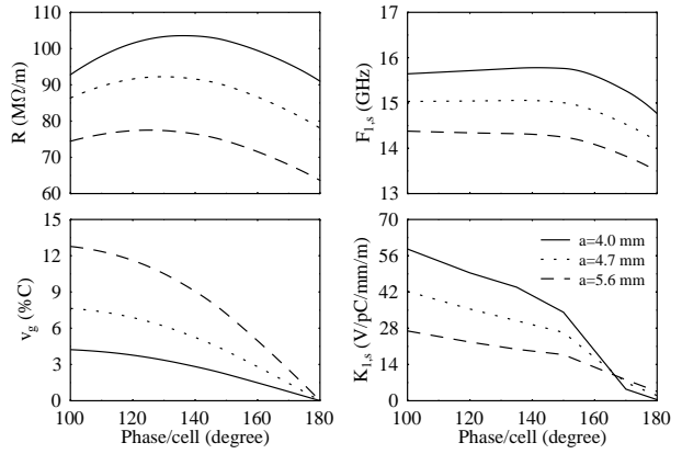
Figure 3 RF parameters v.s. phase advance for three aperture openings at X-band
