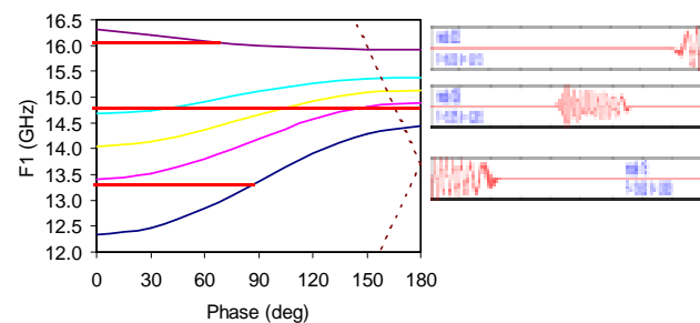
Figure 1 Dipole dispersion and typical modes in a traveling wave structure.
