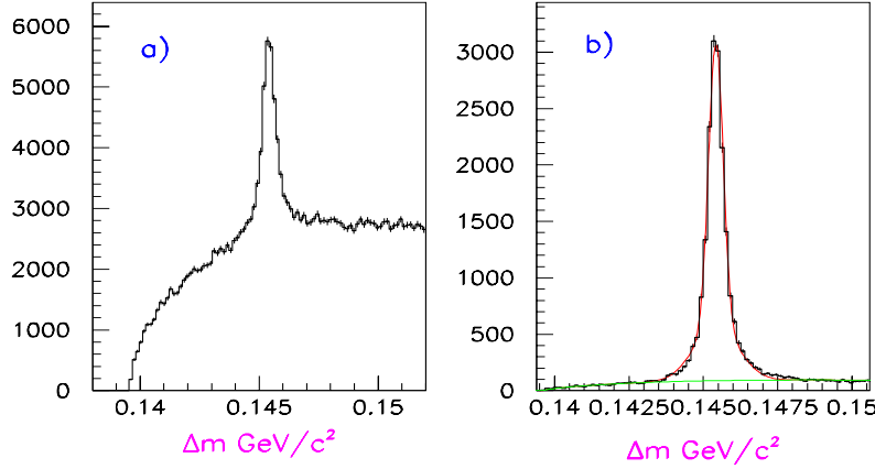
Figure 3: \Delta m distributions for K_S^0 \pi^+ \pi^- a) before and b) after a D^0 mass cut at 2.5\sigma .
