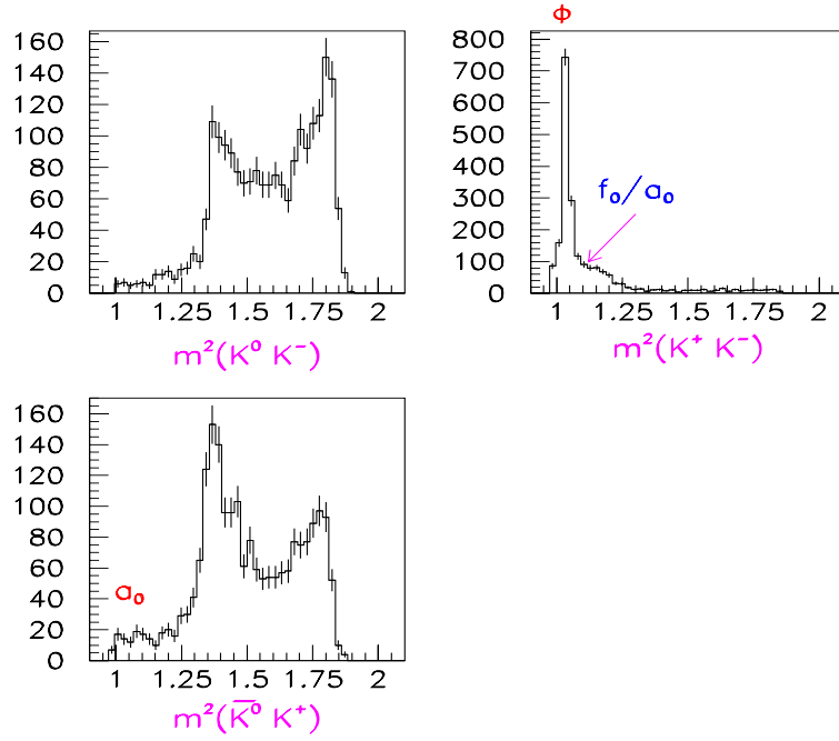
Figure 13: D^0 \rightarrow \bar{K}^0 K^+ K^- Dalitz plot projections.
