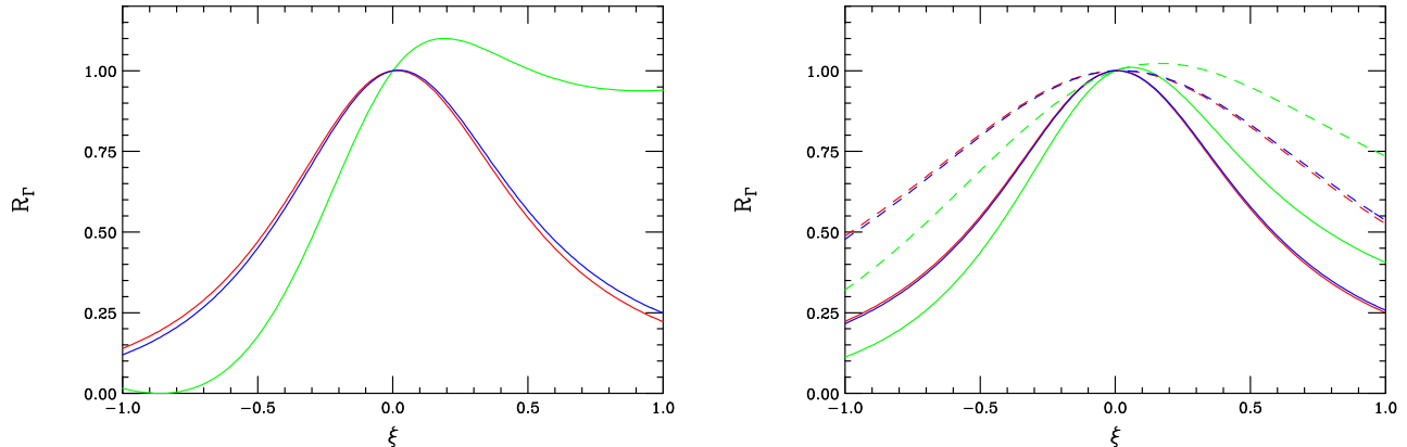
FIG. 4: Ratio of Higgs widths to their SM values, R_\Gamma , as a function of the mixing parameter \xi assuming a Higgs mass of 125 GeV: red for fermion pairs or massive gauge boson pairs, green for gluons and blue for photons. In the left panel we assume a radion mass m_r = 300 GeV and v/\Lambda = 0.2 . In the right panel the solid (dashed) curves are for m_r = 500 (300) GeV and v/\Lambda = 0.2 (0.1).
