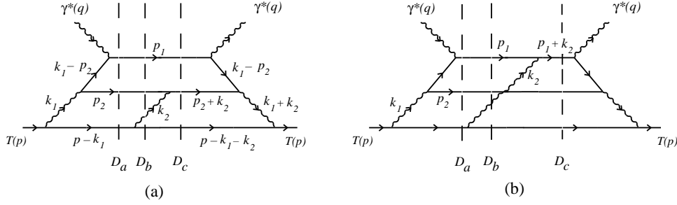
FIG. 3: Two types of final state interactions. (a) Scattering of the antiquark ( p_2 line), which in the aligned jet kinematics is part of the target dynamics. (b) Scattering of the current quark ( p_1 line). For each LC time-ordered diagram, the potentially on-shell intermediate states – corresponding to the zeroes of the denominators D_a, D_b, D_c – are denoted by dashed lines.
