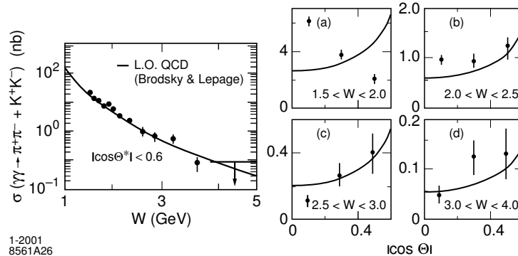
FIG. 1: Comparison of the sum of \gamma\gamma \rightarrow \pi^+\pi^- and \gamma\gamma \rightarrow K^+K^- meson pair production cross sections with the scaling and angular distribution of the perturbative QCD prediction [73]. The data are from the CLEO collaboration [81].
