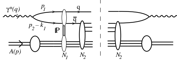
FIG. 2: Glauber-Gribov shadowing involves interference between rescattering amplitudes.
