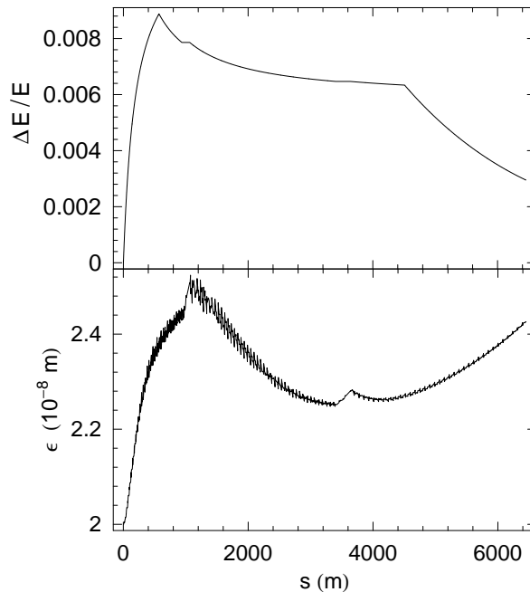
Figure 8: Correlated energy spread for BNS damping (top) and vertical emittance growth in the beam for an initial offset of 2\text{ }\mu\text{m} (bottom).
