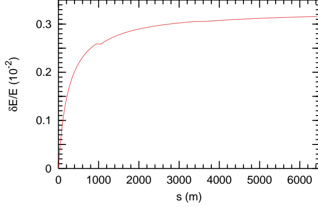
Figure 10: Energy spread in the beam for RF phase of -10.9 degrees.
