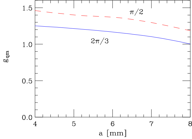
Figure 6: Cylindrically symmetric, disk-loaded structure operated in a quadrupole ( m = 2 ) mode: the relative (compared to the normal MQ structure) strength factor g_{qm} vs. iris radius a . For the normal MQ structure we take \eta = 0.8 and R_s to be 25% less than that of the cylindrically symmetric model.
