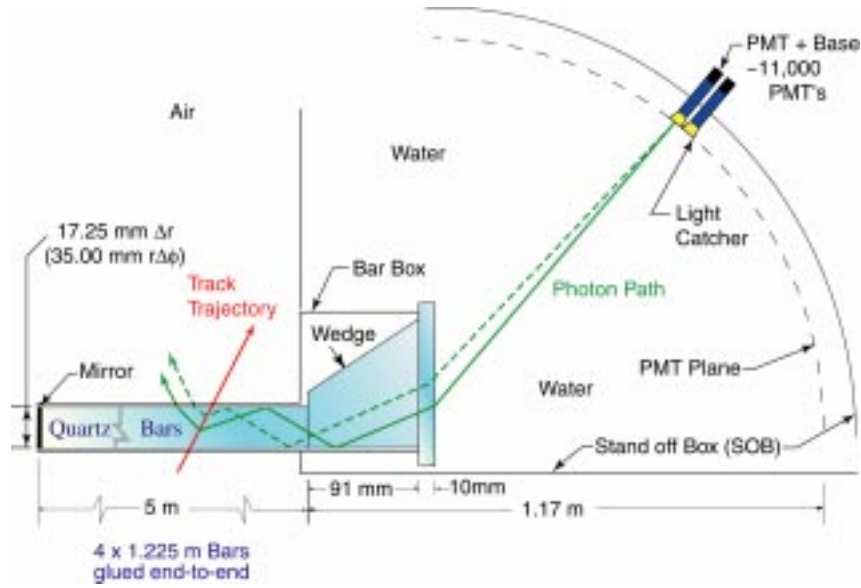
Figure 3: The principle of the DIRC; incident charged particles emit Cherenkov radiation as they pass through the quartz bars. The Cherenkov photons are reflected to the end of the quartz bar and out in a water tank, which is instrumented with photomultipliers to detect the light.
