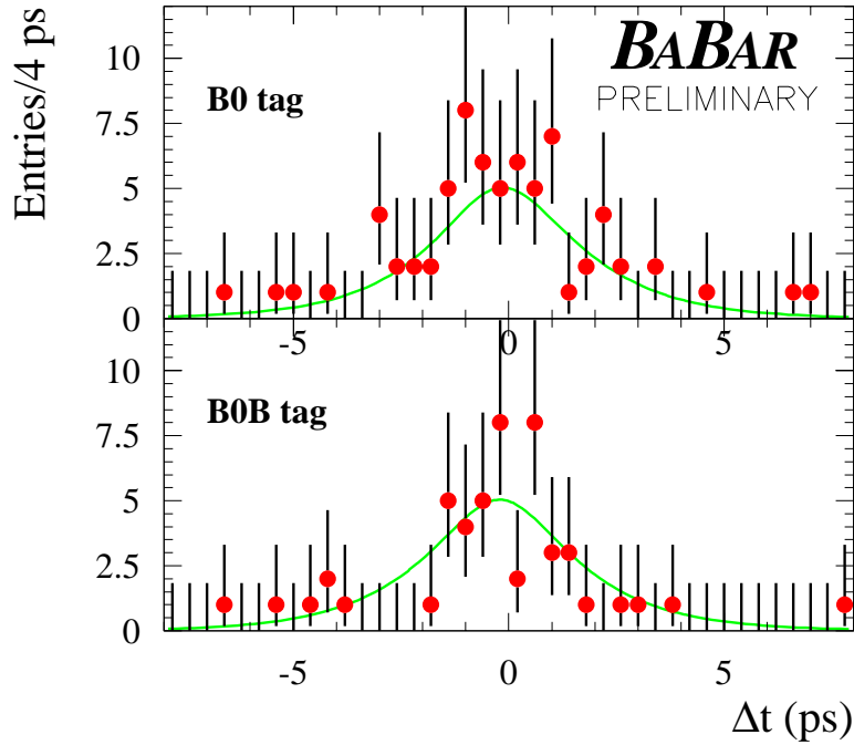
Figure 8: The \Delta t distributions for events in the CP sample tagged as B^0 and \bar{B}^0 respectively. The asymmetry in the number of B^0 and \bar{B}^0 tags are apparent in the plot. The shift to negative values of \Delta t is due to the small bias, about 0.2 ps, in the time resolution.
