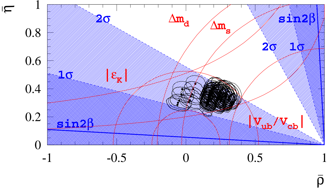
Figure 10: The constraints in the \hat{\rho} - \hat{\eta} planes, and the result of our determination of \sin 2\beta overlaid. The following measurements are used: |V_{cb}| = 0.0402 \pm 0.017 , |V_{ub}/V_{cb}| = \langle |V_{ub}/V_{cb}| \rangle \pm 0.0079 , \Delta m_{B_d} = 0.472 \pm 0.017 \text{ hps}^{-1} and |\epsilon_K| = (2.271 \pm 0.017) \times 10^{-3} , and for \Delta m_{B_s} the set of amplitudes corresponding to a 95%CL limit of 14.6 \text{ hps}^{-1} . We scan the model-dependent parameters \langle |V_{ub}/V_{cb}| \rangle , B_K , f_{B_d} \sqrt{B_{B_d}} and \xi_s , in the range [0.070, 0.100] , [0.720, 0.980] , [185, 255] \text{ MeV} and [1.07, 1.21] , respectively. \sin 2\beta = 0.12 \pm 0.37(\text{stat}) is represented by cross-hatched regions corresponding to one and two statistical standard deviations.
