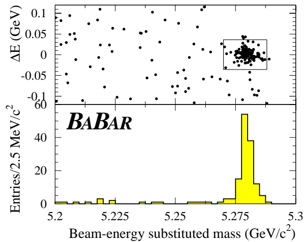
Figure 4: The signal in the B^0 \rightarrow J/\psi K_S^0 , K_S^0 \rightarrow \pi^+ \pi^- mode.
