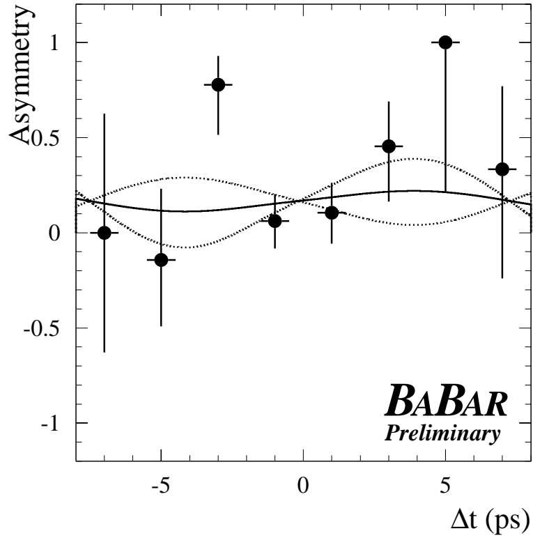
Figure 9: The raw B^0 - \bar{B}^0 asymmetry (N_{B^0} - N_{\bar{B}^0})/(N_{B^0} + N_{\bar{B}^0}) , with binomial errors, as a function of \Delta t . The solid line is the asymmetry for our central value of \sin 2\beta . The dotted lines represents one statistical standard deviations from the central value.
