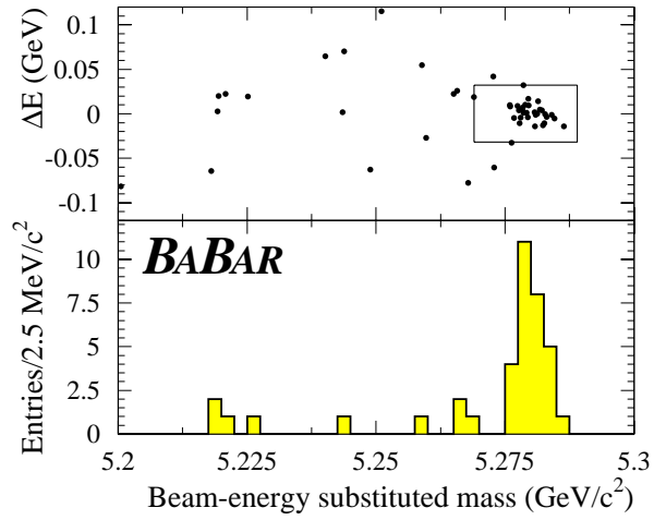
Figure 6: The signal in the B^0 \rightarrow \psi(2S) K_S^0, K_S^0 \rightarrow \pi^+ \pi^- mode.
