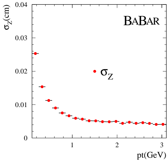
Figure 2: The impact parameter resolution in z for the silicon vertex tracker as measured by cosmic muons.
