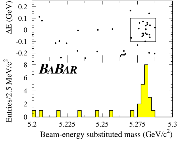
Figure 5: The signal in the B^0 \rightarrow J/\psi K_S^0, K_S^0 \rightarrow \pi^0 \pi^0 mode.
