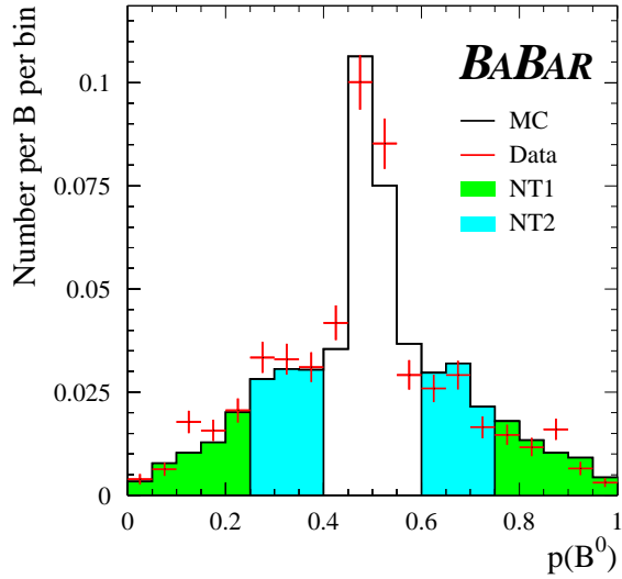
Figure 7: The output from the neural network for B flavor tagging. The data is shown as points with error bars and the histogram shows the Monte Carlo. Events close to 1 (0) are likely to be B^0 ( \bar{B}^0 ) tags. Events near 0.5 provide no tagging information and are not used.
