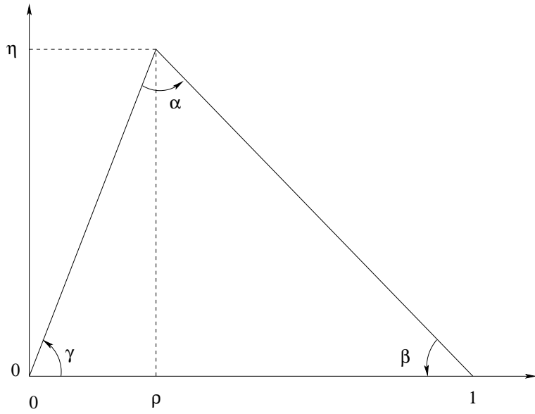
Figure 1: The CKM triangle formed by unitarity between the first and third generation. The study of time dependent asymmetry in B^0 \rightarrow J/\psi K_S^0 allows us to determine \sin 2\beta .
