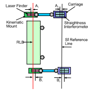
Fig. 2 Alignment jig
