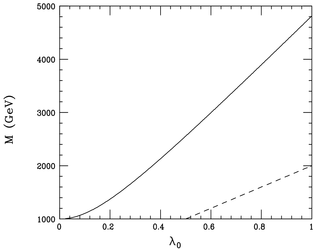
Figure 6: Same as Fig. 1 but now for s -channel \tilde{\nu} exchange. Here \lambda_0^2 equals the product of the relevant Yukawa couplings in the superpotential. The typical region excluded by low energy data is that below the dashed curve in the lower right hand corner.
