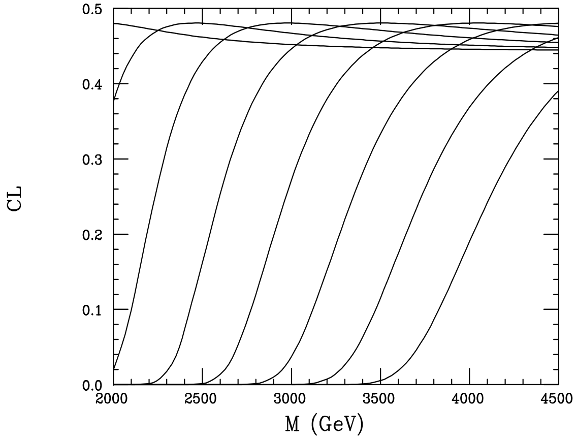
Figure 7: Average confidence level of the best fit to the parameters A and B as a function of the \tilde{\nu} mass in the case of s -channel \tilde{\nu} exchange for various values of the Yukawa coupling \lambda_0 in the range 0.3 to 1.0 in steps of 0.1 from top left to lower right.
