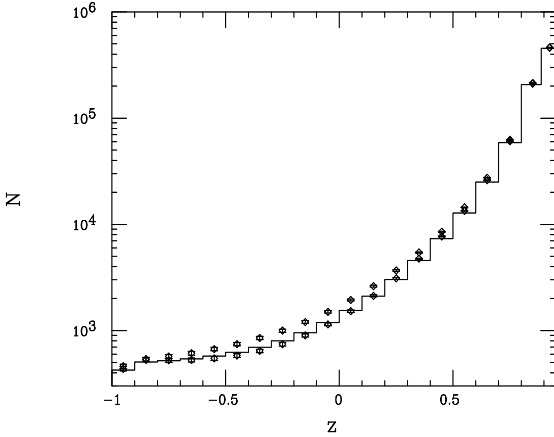
Figure 11: Same as the previous figure but now for a 3 TeV Z' in comparison to the SM. The upper(lower) set of data points corresponds to g_L^{e'} = g_R^{e'} = 0.5c ( g_L^{e'} = -g_R^{e'} = 0.5c ).
