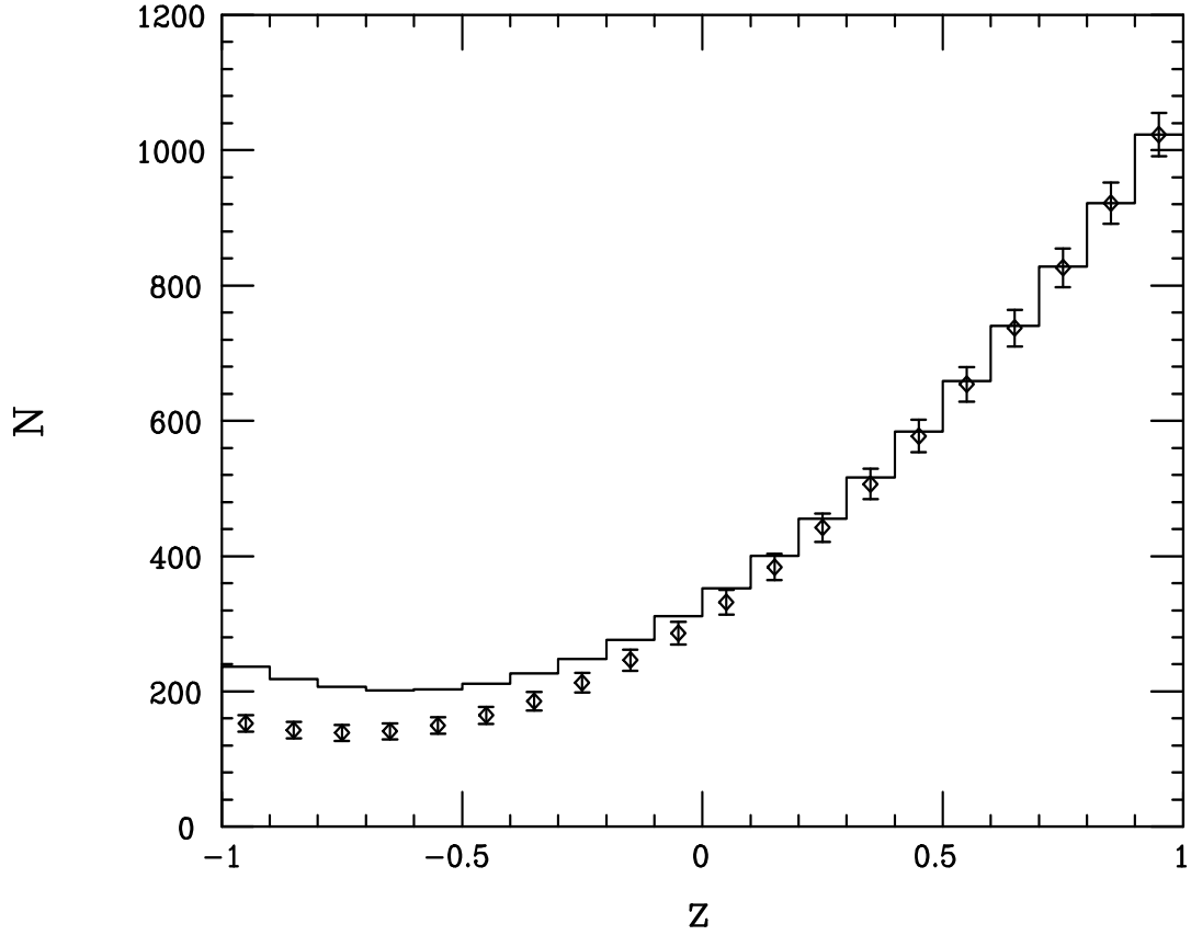
Figure 2: Binned angular distribution for the process e^+e^- \rightarrow \mu^+\mu^- or \tau^+\tau^- at a 1 TeV NLC in the SM (histogram) and for the case where a 3 TeV \tilde{\nu} with \lambda = 0.5 exchanged in the t -channel also contributes. The errors are statistical only and represent an integrated luminosity of L = 150 \text{ fb}^{-1} . Initial state radiation has been included.
