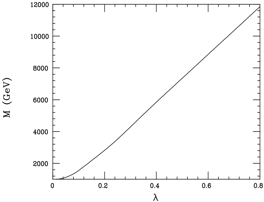
Figure 1: Indirect search reach for t -channel exchanged \tilde{\nu} 's as a function of their mass from the process e^+e^- \rightarrow \mu^+\mu^- or \tau^+\tau^- at a 1 TeV NLC with an integrated luminosity of L = 150 \text{ fb}^{-1} including the effects of initial state radiation. The discovery region lies below the curve.
