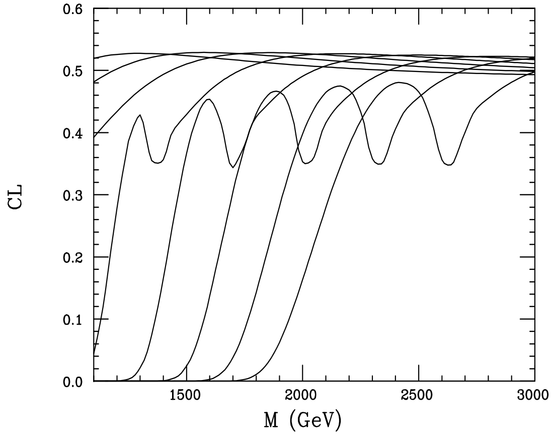
Figure 5: Average confidence level of the best fit to the parameters A and B as a function of the \tilde{\nu} mass in the case of t -channel \tilde{\nu} exchange for various values of the Yukawa coupling \lambda in the range 0.3 to 1.0 in steps of 0.1 from top left to lower right.
