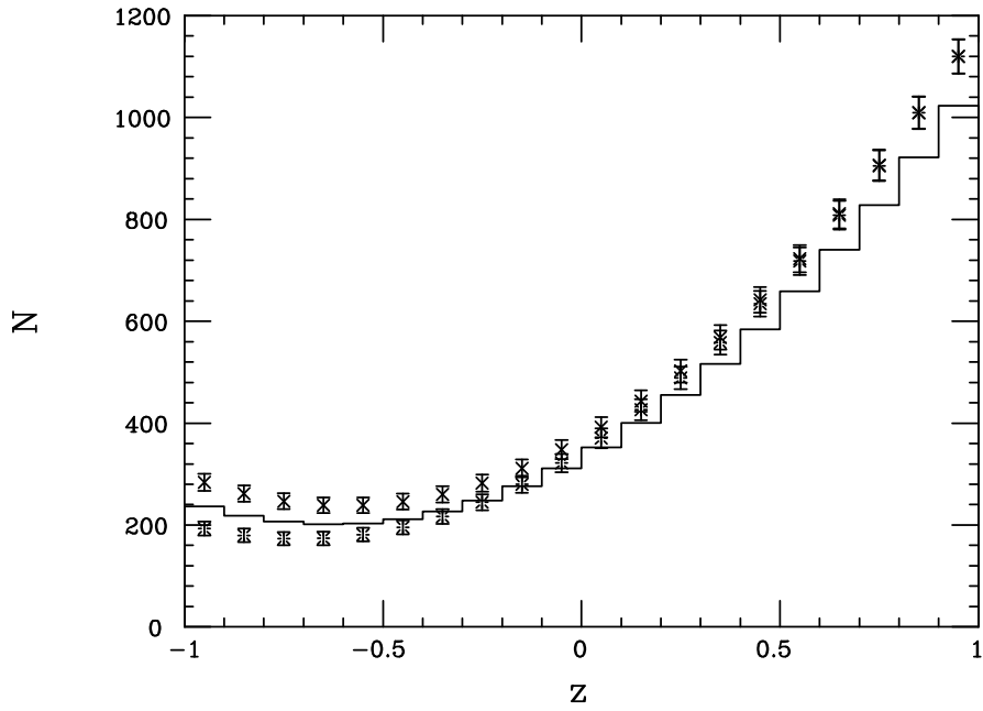
Figure 3: Same as the previous figure but now including a 3 TeV Z' exchange in the s -channel. The magnitude of all Z' couplings is taken to be the same value, i.e. , |g_{L,R}^{e,f'}| = 0.3c , for purposes of demonstration. In the top panel, the relative signs of (g_L^e, g_R^e, g_L^{f'}, g_R^{f'}) are chosen to be (+, -, +, -)[(+, +, +, +)] for the upper[lower] series of data points, while in the bottom panel they correspond to the choices (+, -, -, +)[(+, +, -, -)] for the upper[lower] series, respectively.
