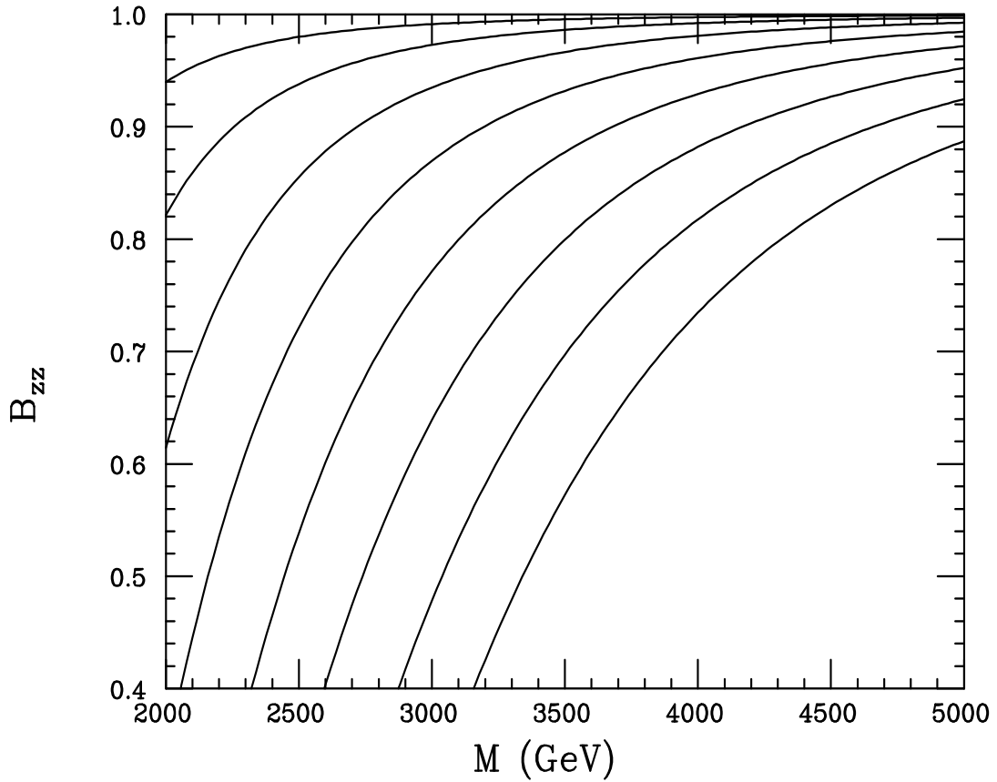
Figure 8: Double \tau spin asymmetry at a 1 TeV NLC as a function of the \tilde{\nu} mass for different values of the Yukawa coupling \lambda_0 . From left to right, \lambda_0 varies from 0.3 to 1.0 in steps of 0.1 as in the previous figure. In the case of either the SM or a Z' , B_{zz} = 1 .
