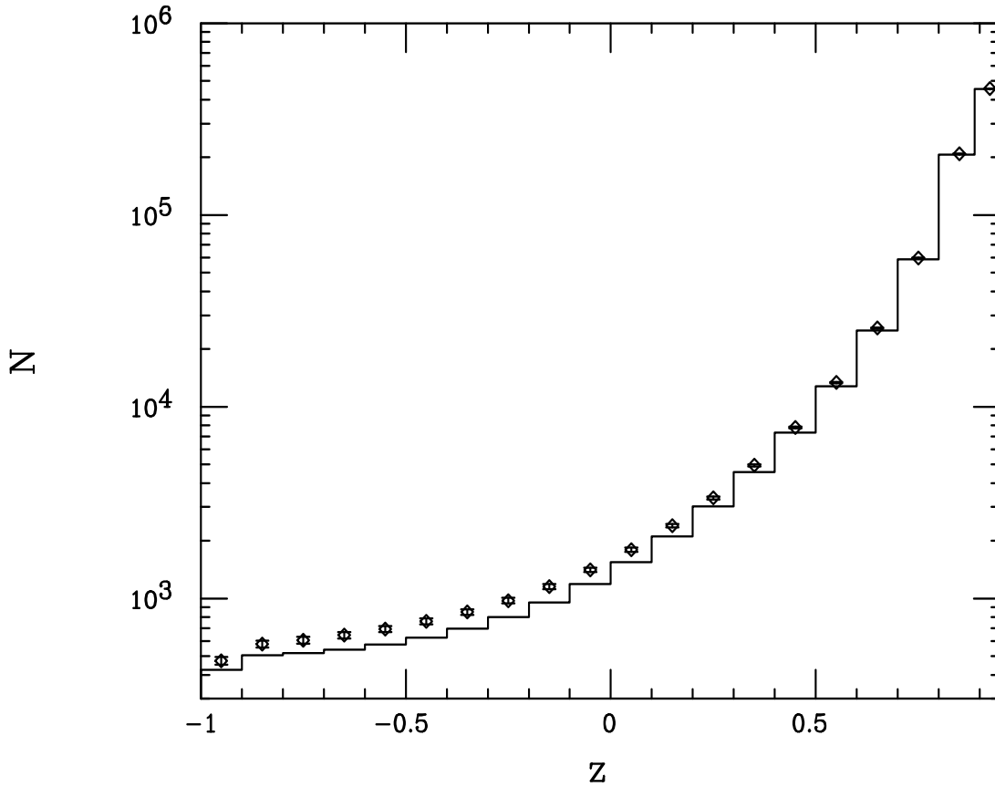
Figure 10: Same as Fig.2 but now for the case of Bhabha scattering. Angular cuts as described in the text have been employed to render the cross section finite in the forward direction.
