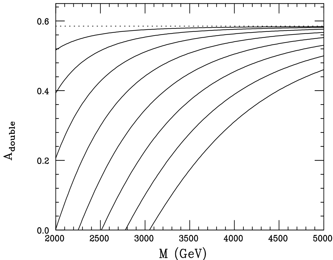
Figure 9: The double polarization asymmetry, A_{double} as a function of the \tilde{\nu} mass at a 1 TeV NLC for different choices of \lambda_0 . From left to right, \lambda_0 varies from 0.3 to 1.0 in steps of 0.1. The dotted curve corresponds to the value obtained for both the SM and in the case of a Z' .
