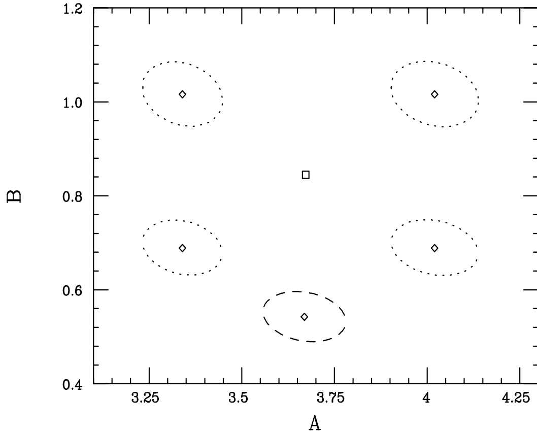
Figure 4: 95% CL fits to the values of A and B for the data generated with \tilde{\nu} exchange (dashed region) and for the data generated for the four possible choices of Z' couplings (dots). The SM result is represented by the square in the center of the figure while the diamonds are the locations of the best fits.
