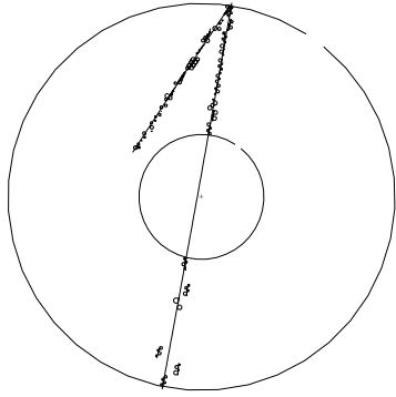
Figure 2: View of a cosmic ray from commissioning of the BaBar drift chamber. Approximately 50% of the chamber is instrumented; the gaps in the lower track and the termination in the track away from the IP are due to uninstrumented regions. The stereo hits are plotted at wire center, hence deviations from the fitted tracks indicate z position. The tracks are drawn as reconstructed by the reconstruction software – the track through the IP is actually reconstructed as two tracks.
