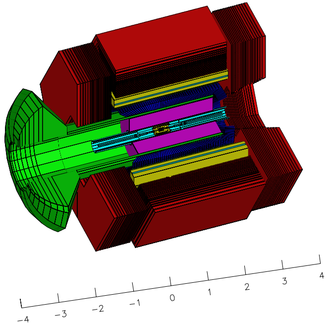
Figure 1: Cut-away view of the BaBar detector, as seen by the simulation program. The scale is in meters. At smallest radii are the PEP-II beam components and silicon vertex tracker, followed by the drift chamber and the DIRC quartz bars. Outside the DIRC is the CsI calorimeter, followed by cylindrical RPCs, the solenoid coil, and the instrumented flux return. The large object at the left is the water stand-off box for the DIRC.
