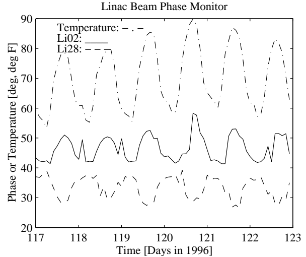
Figure 4: Beam phase in sector 2 and 28 and outside temperature showing an anticorrelation and a phase variation of 7^\circ . The temperature swing during that period was about 28^\circ\text{F} daily.
