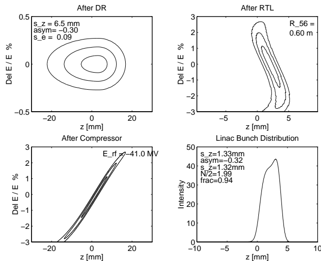
Figure 1: Bunch Compression Setup.
