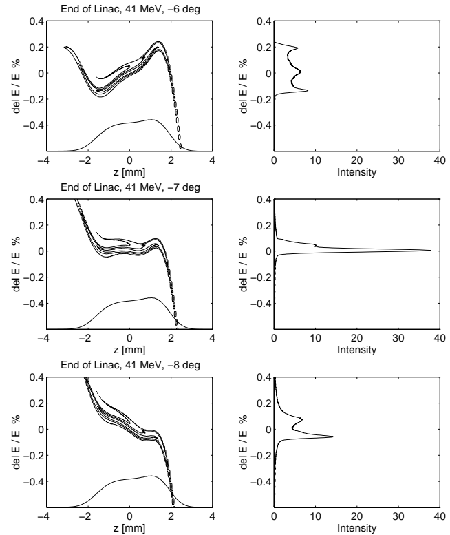
Figure 2: Energy-z correlation for different linac phase. Small phase changes of \pm 1^\circ influence the energy-z correlation which changes the IP bunch length by 20%. The beam distribution is generated by over-compression. The lower plots show the energy distribution on the right.
