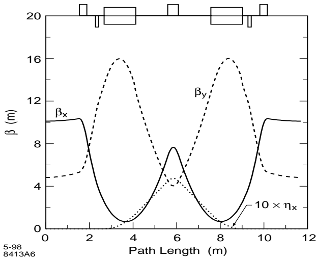
Figure 2: SPEAR 3 Main Cell Optics.
