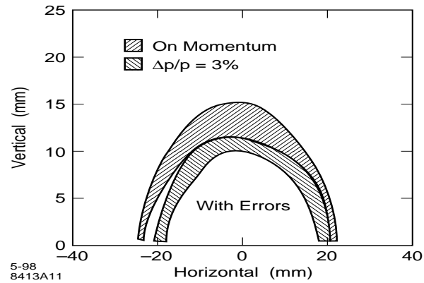
Figure 4: Dynamic Aperture with Errors
