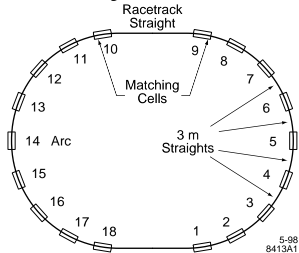
Figure 1: Layout of the SPEAR magnet girders.
