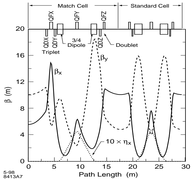
Figure 3: SPEAR 3 Matching Cell Optics.
