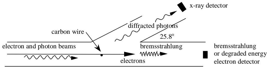
FIGURE 3. Combined electron/photon beam position monitor for one plane. Both beams strike the carbon wire; when they overlap, detectors record maximum signals simultaneously.
