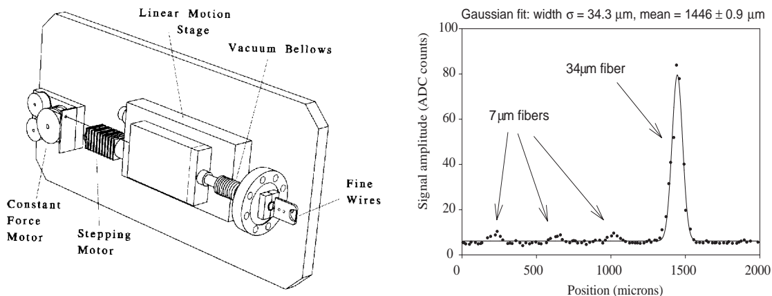
FIGURE 2: Wire scanner with micron resolution beam profile and centroid measurement (SLAC).
