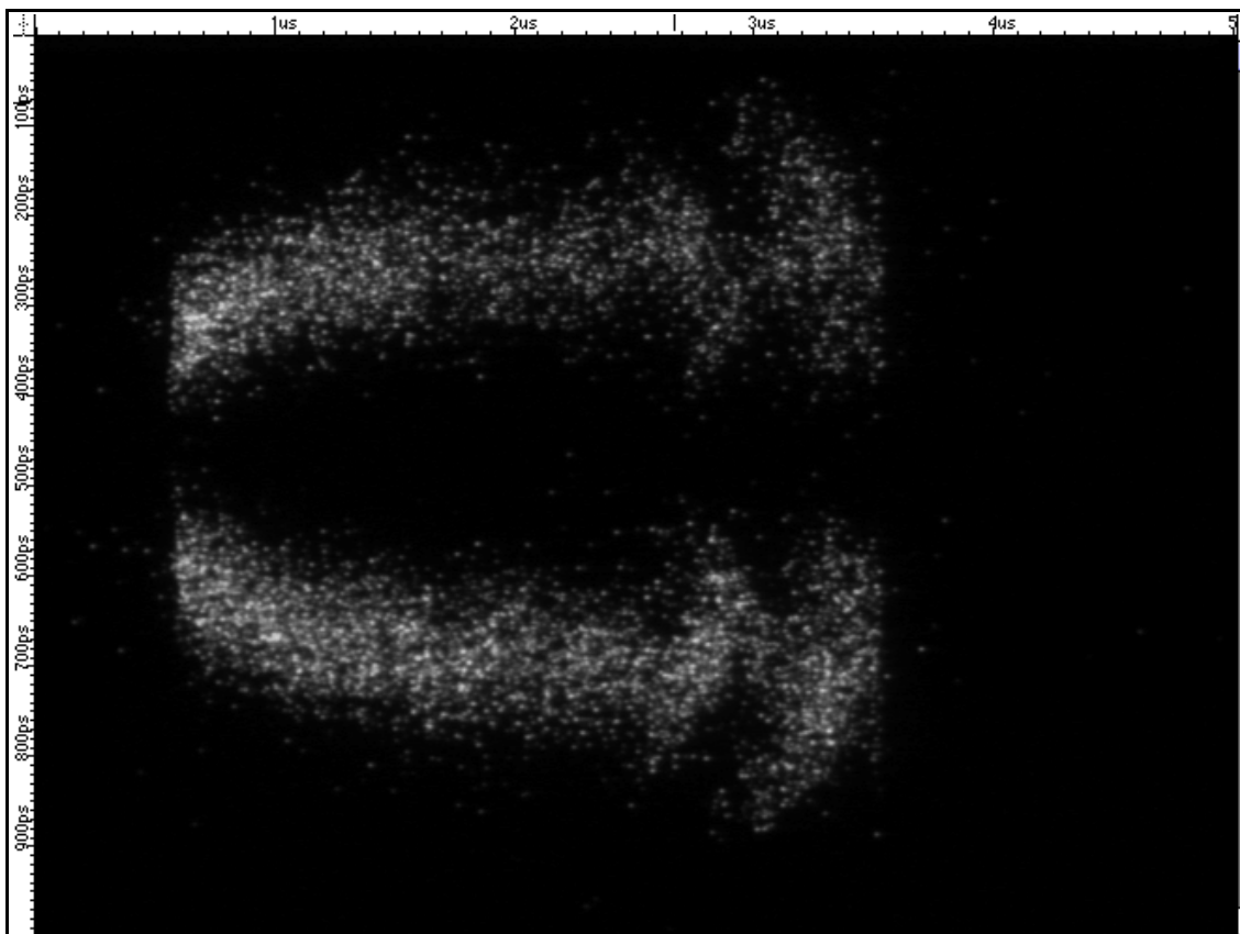
FIGURE 6. Large longitudinal oscillations at the end of a 700-bunch train with a 228 mA current and 4.2-ns spacing. Full scale: 1 ns vertical, 5 \mu s horizontal.
