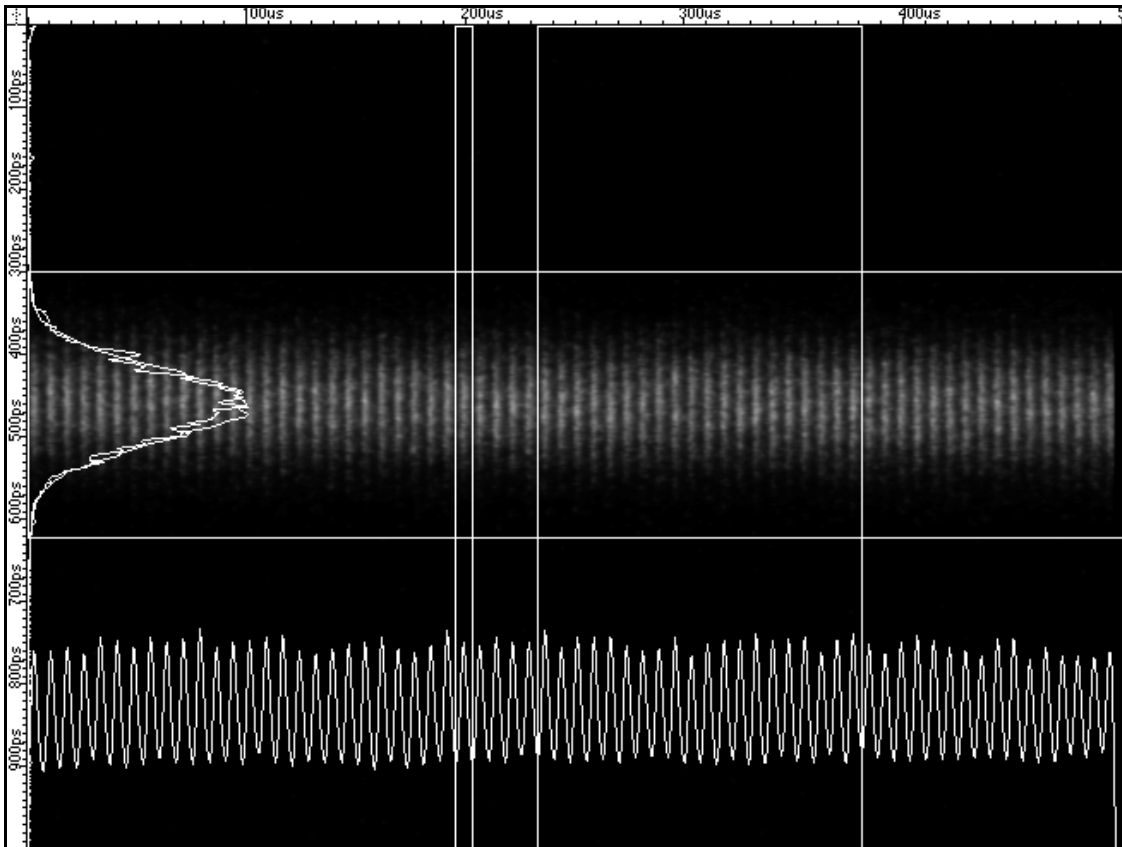
FIGURE 2. The light from a single bunch captured on consecutive turns. Full scale: 1 ns vertical, 500 \mu s horizontal. The projections on the left show a single bunch and the sum of the 20 bunches (determined by the two sets of cursors).
