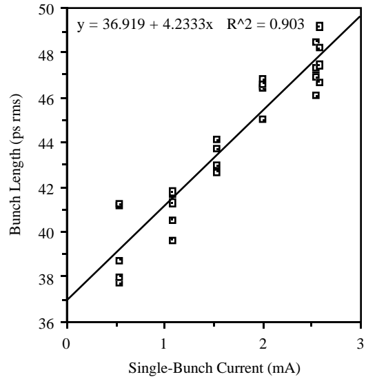
FIGURE 4. Variation of bunch length with single-bunch current, at 14 MV of RF; 1-mA corresponds to 4.6 \times 10^{10} electrons in the bunch.
