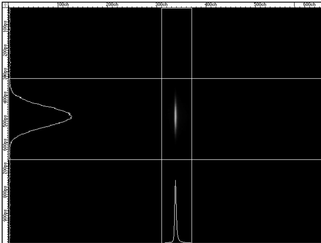
FIGURE 1. Typical single-axis streak image for bunch-length measurements, accumulated over many turns. Vertical: 1 ns full scale. Horizontal: position (channel number) along slit. The projections onto the axes, in the regions bounded by cursors, are shown along the sides.
