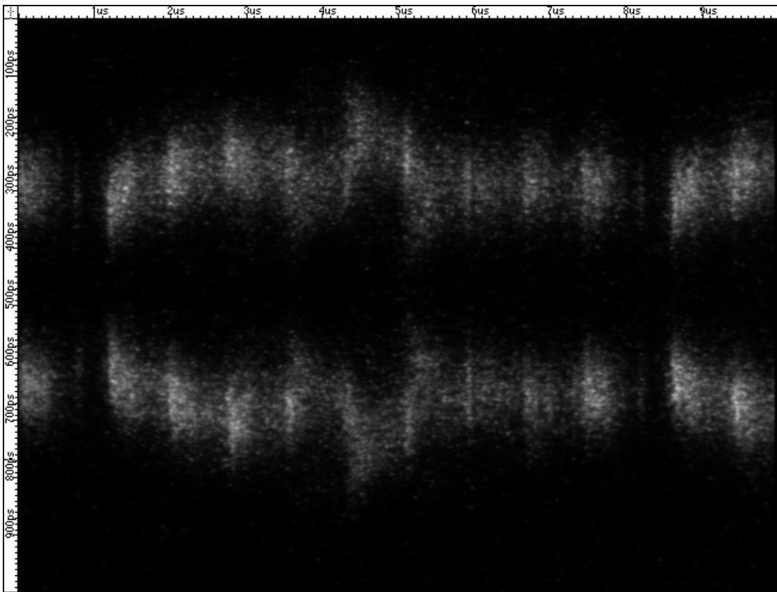
FIGURE 5. Longitudinal instability in the center of a 1658-bunch train with a 480-mA current. Filled in a 9-zone pattern with 4.2-ns spacing and a 5% gap. Full scale: 1 ns vertical, 10 \mu s horizontal.
