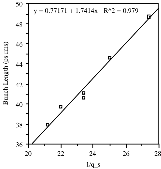
FIGURE 3. Variation of bunch length with the inverse of the synchrotron tune, for a single bunch at 1 mA.
