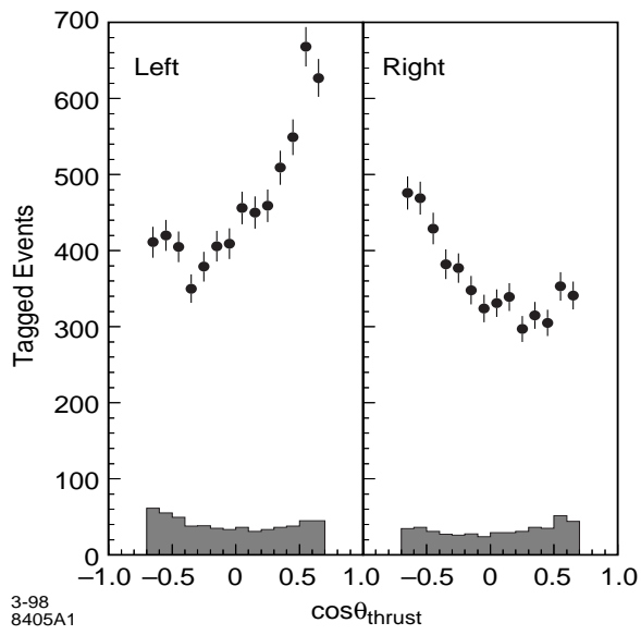
Figure 1: The polar angle distribution of the signed thrust axis for the b tagged sample. The estimated background is shown by the shaded histogram.
