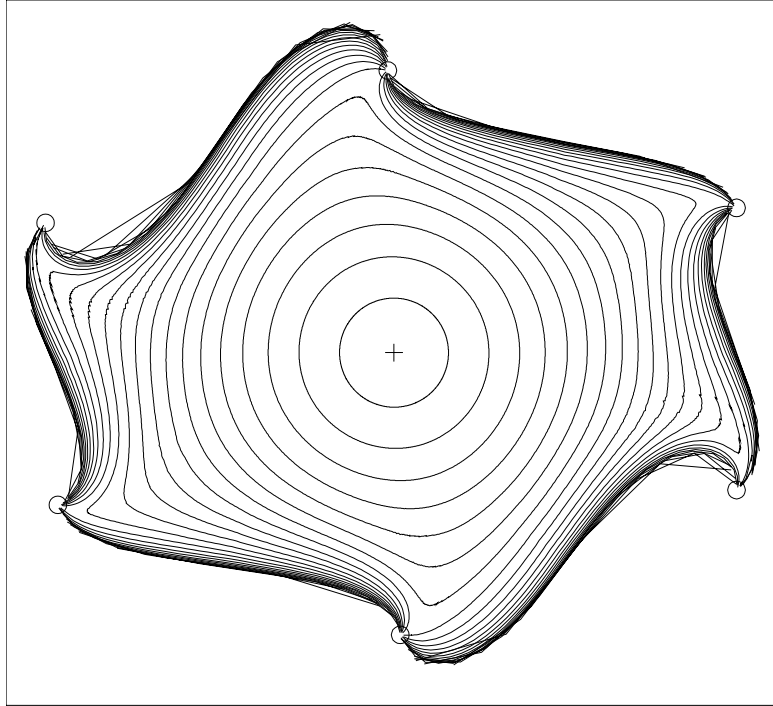
Fig. 3. 50 ns isochrones in a typical BaBar drift chamber cell.
