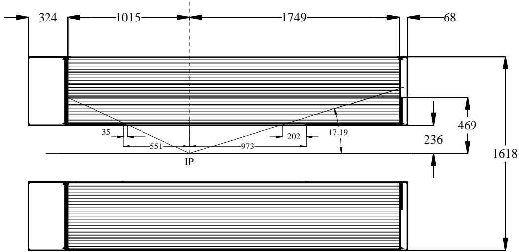
Fig. 1. Side view of the BaBar drift chamber. The dimensions are expressed in mm.
