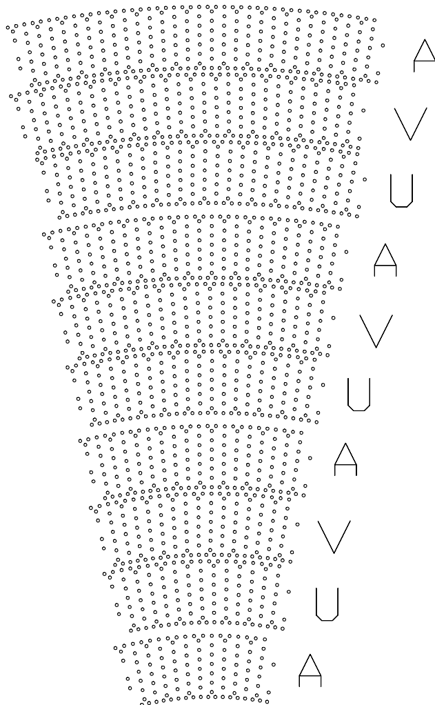
Fig. 2. Cell layout in the BaBar Drift Chamber.
