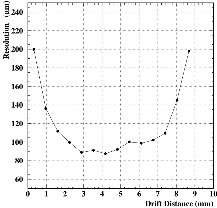
Fig. 4. Spatial resolution obtained in the Prototype drift chamber with sense wire voltage at 2020 V.
