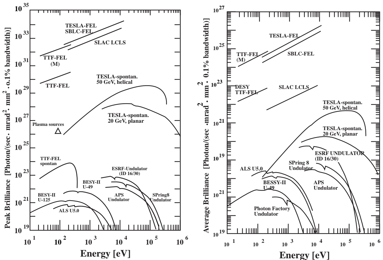
Figure 2a, 2b; Peak and average source brightness as a function of photon energy for short wavelength FELs in comparison with synchrotron radiation sources and conventional X-ray generators. Courtesy of J. Rossbach, DESY.
