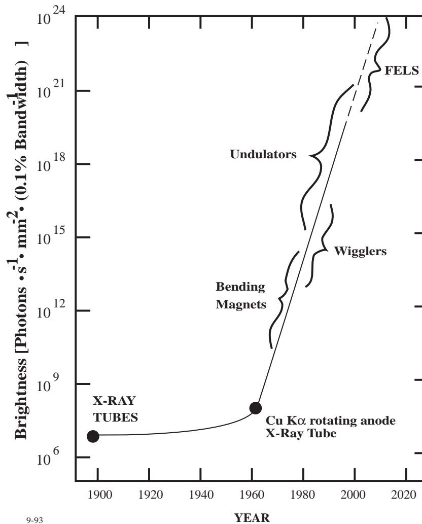
Figure 1: X-ray source brightness as a function of time since the discovery of X-rays in 1895.
