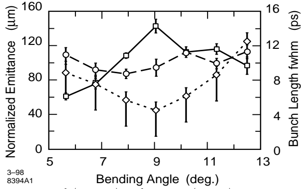
FIG. 1. Measured rms normalized horizontal (squares) and vertical (circles) emittances and rms bunch length (diamonds) versus angle in the 1st bend of the compressor with 6nC.
