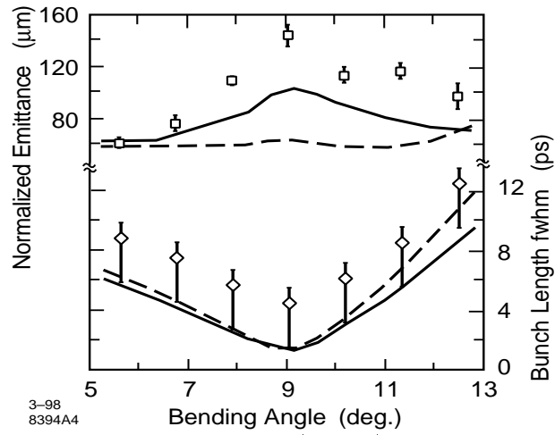
FIG. 4. Comparison of the measured rms horizontal emittance (squares) and rms bunch length (diamonds) with PARMELA (dashes) and CSR-TRACK (solid) for 6nC per bunch.
