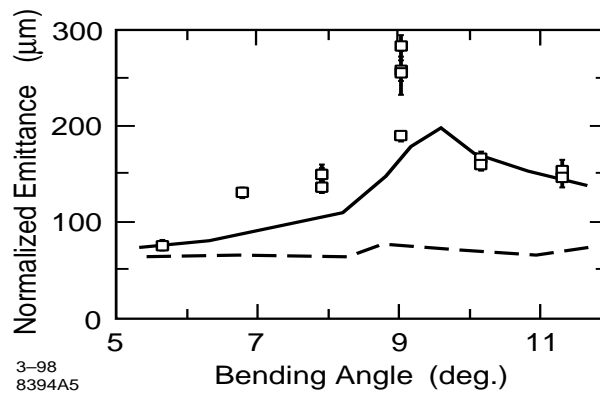
FIG. 5. Comparison of the measured rms horizontal emittance (squares) with PARMELA (dashes) and CSR-TRACK (solid) for 16nC per bunch.
