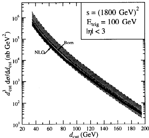
Figure 3: Dependence of the gluonic p\bar{p} \rightarrow 3 jet cross-section on the jet resolution parameter d_{\text{cut}} for the k_T clustering algorithm. 6 The gray and black bands result from varying the renormalization/factorization scale \mu over the range d_{\text{cut}}/2 < \mu < 2d_{\text{cut}} for the Born and NLO results, respectively.
