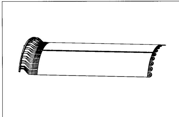
Figure 4: Schematic drawing of two of the eight panels. They contain flattened aluminum tubes through which radioactive fluorinert will circulate in front of the barrel crystals. The liquid enters and exits through the manifold shown on the left side.
