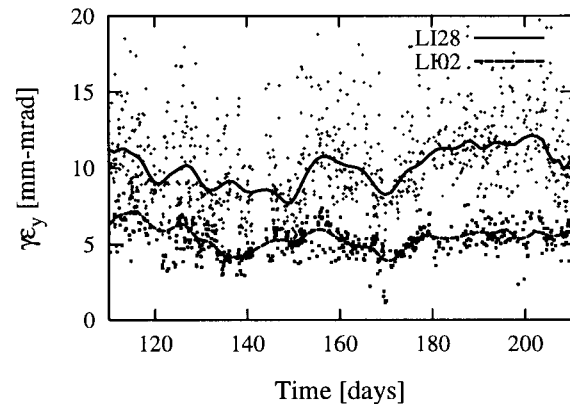
Figure 7 Measured vertical emittances against time for the beginning (LI02) and end (LI28) of the SLAC linac. The data covers the period from April 1 st to July 31 st .
