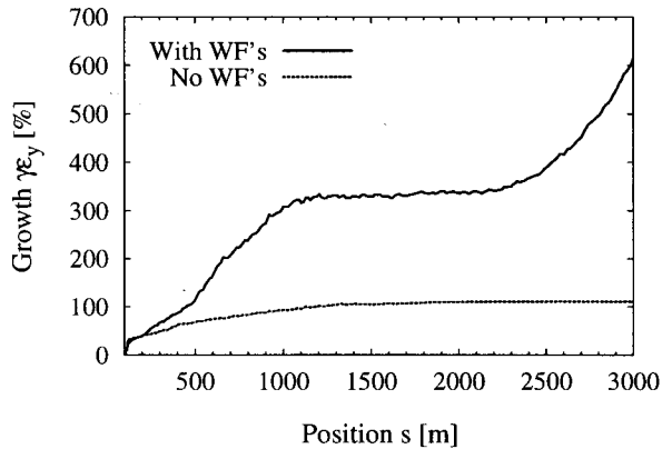
Figure 4 Simulated average vertical emittance along the linac for flat trajectories, with and without wakefields.
