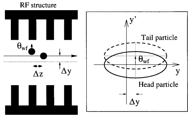
Figure 1 Principle of a wakefield generated increase in the projected emittance. A single bunch is represented by two longitudinal slices (particles). The projected beam emittance is increased due to a wakefield kick \theta_{\text{WF}} .
