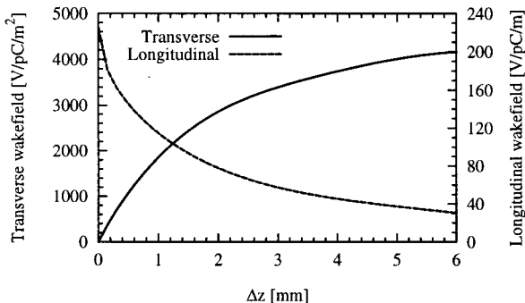
Figure 2 Calculated transverse and longitudinal wakefield functions for the SLC [1].
