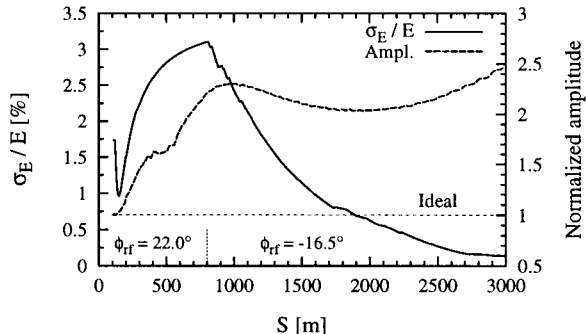
Figure 3 Simulated energy spread and normalized amplitude of a betatron oscillation along the SLAC linac.
