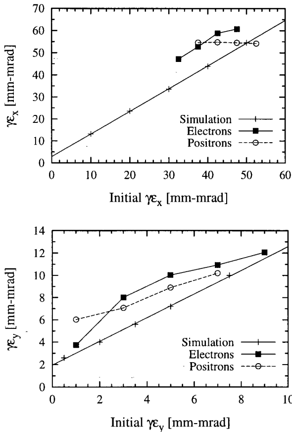
Figure 8 Normalized horizontal and vertical emittances at the end of the linac (sector 28) versus the initial emittances. Simulation results for electrons are compared to the electron and positron average measurements during the 1996 run. Statistical errors are too small to be visible.
