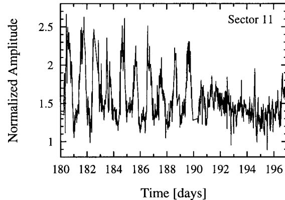
Figure 9 Variation of the normalized amplitude of an incoming betatron oscillation in the middle of the SLAC linac. A fix was applied on day 191 [5].
