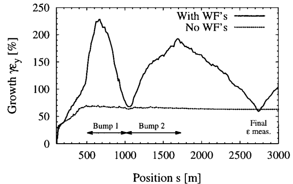
Figure 6 Simulated average vertical emittance along the linac after bump optimization.
