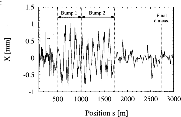
Figure 5 Horizontal linac trajectory with bumps during record luminosity on June 21 st .
